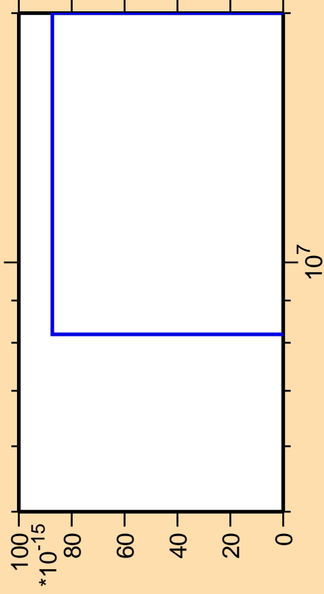
\Delta\sigma/\sigma vs. E for ^{213}\text{Ra}(\text{mt } 42)
