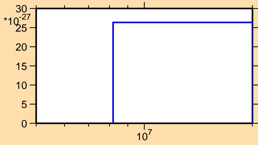
\sigma vs. E for ^{213}\text{Ra}(\text{mt } 42)
