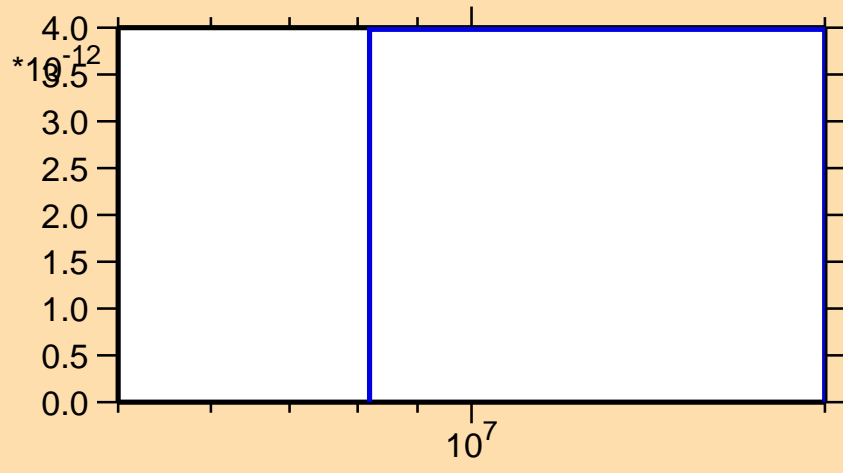
\sigma vs. E for ^{213}\text{Ra} (mt 34)
