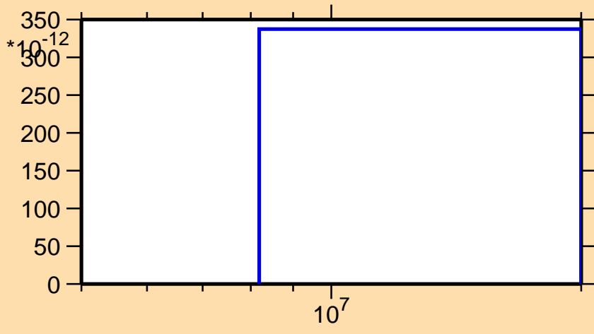
\sigma vs. E for ^{213}\text{Ra}(n,\text{pd})
