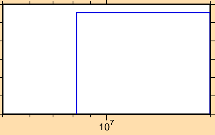
\sigma vs. E for ^{213}\text{Ra}(n,2np)
