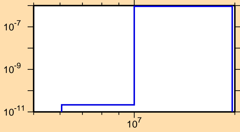
\sigma vs. E for ^{214}\text{Ra} (mt 45)
