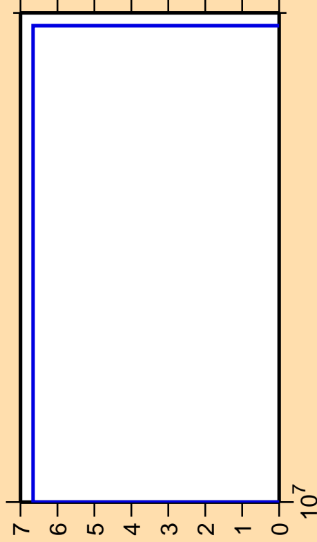
\Delta\sigma/\sigma vs. E for ^{214}\text{Ra}(n,\text{pt})
