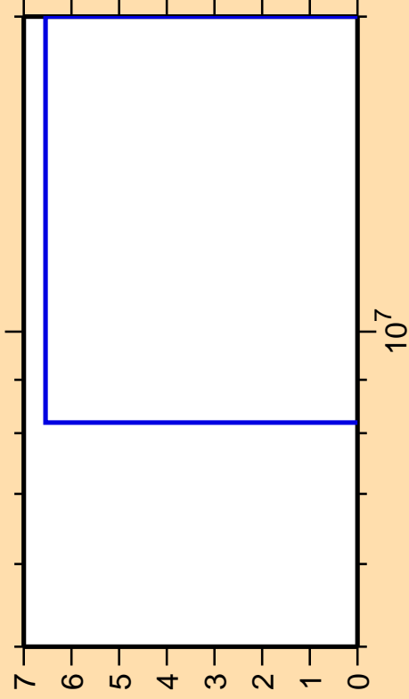
\Delta\sigma/\sigma vs. E for ^{214}\text{Ra}(n,3n\alpha)
