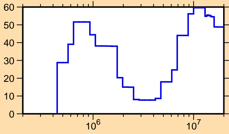
\Delta\sigma/\sigma vs. E for ^{221}\text{Ra}(n,\text{el.})
