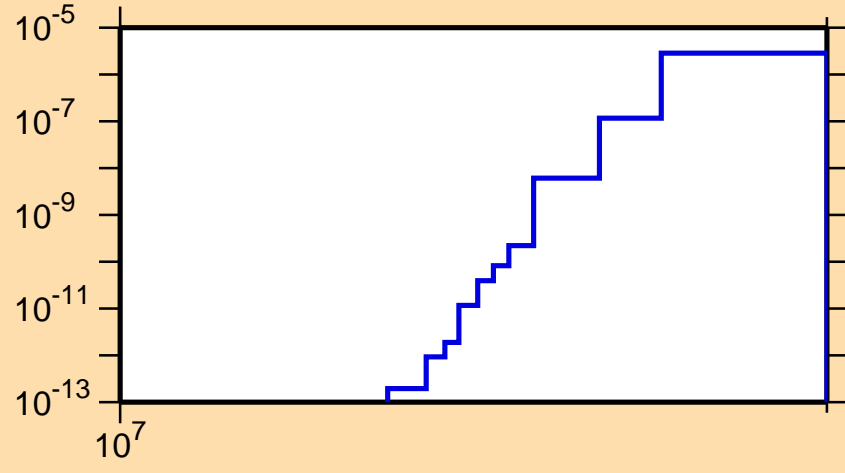
\sigma vs. E for ^{221}\text{Ra}(n,nt)
