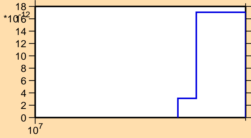
\sigma vs. E for ^{221}\text{Ra} (mt 45)
