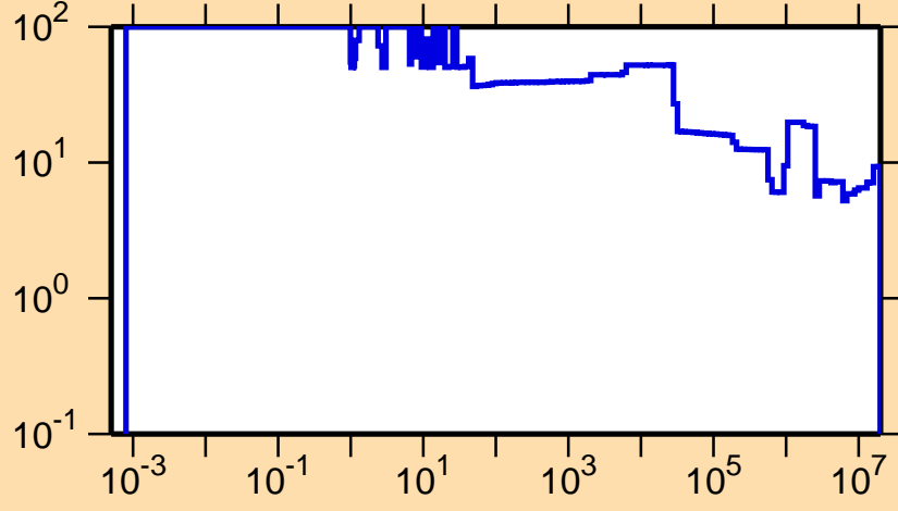
\Delta\sigma/\sigma vs. E for ^{221}\text{Ra}(n,\text{nonel.})
