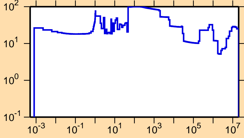
\Delta\sigma/\sigma vs. E for ^{221}\text{Ra}(n,\text{tot.})
