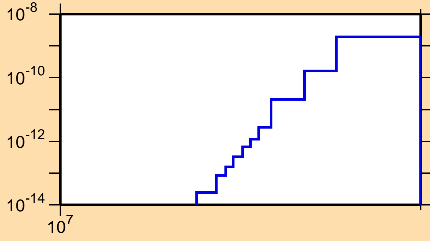
\sigma vs. E for ^{221}\text{Ra}(n,\text{He}3)
