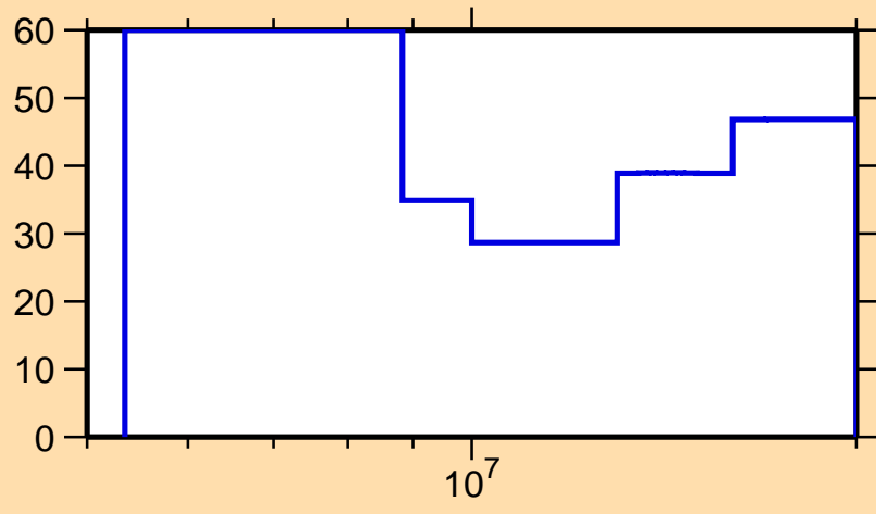
\Delta\sigma/\sigma vs. E for ^{221}\text{Ra}(n,2n)
