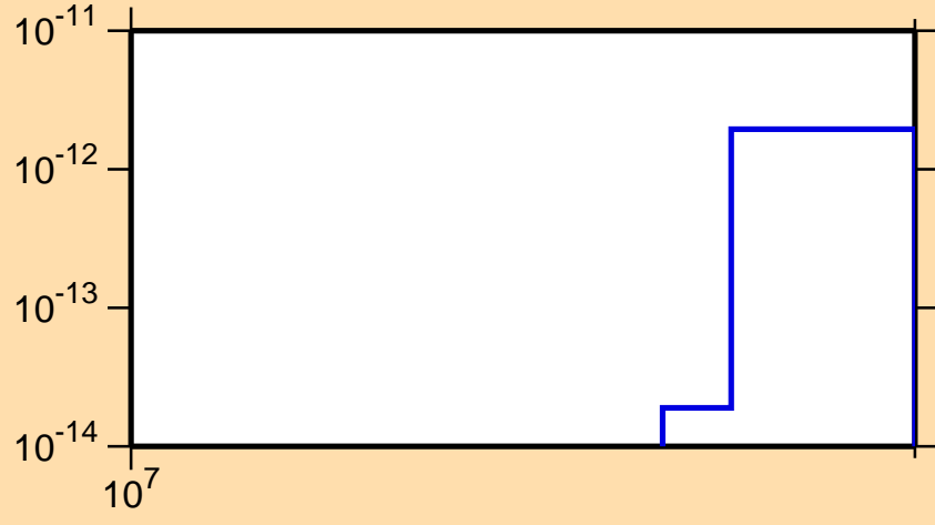
\sigma vs. E for ^{221}\text{Ra} (mt 34)
