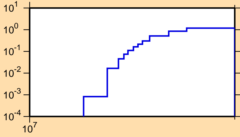
\sigma vs. E for ^{221}\text{Ra}(n,3n)
