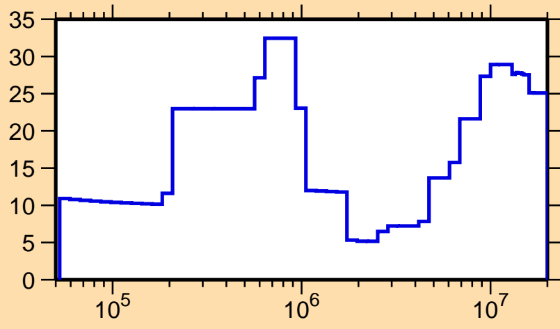
\Delta\sigma/\sigma vs. E for ^{221}\text{Ra}(n,\text{tot.})
