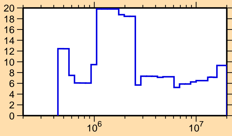
\Delta\sigma/\sigma vs. E for ^{221}\text{Ra}(n,\text{nonel.})
