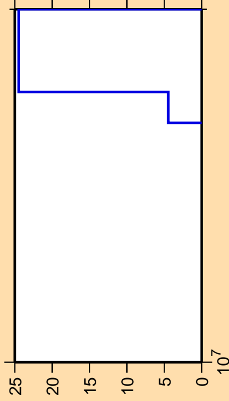
\Delta\sigma/\sigma vs. E for ^{221}\text{Ra} (mt 45)
