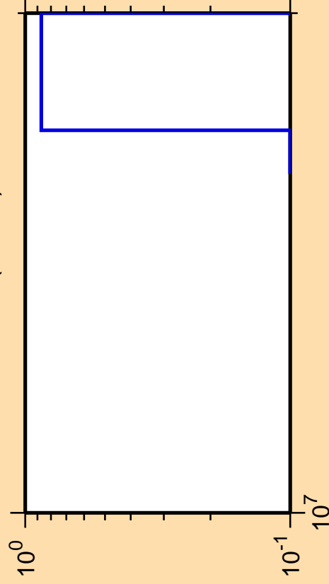
\Delta\sigma/\sigma vs. E for ^{221}\text{Ra} (mt 34)
