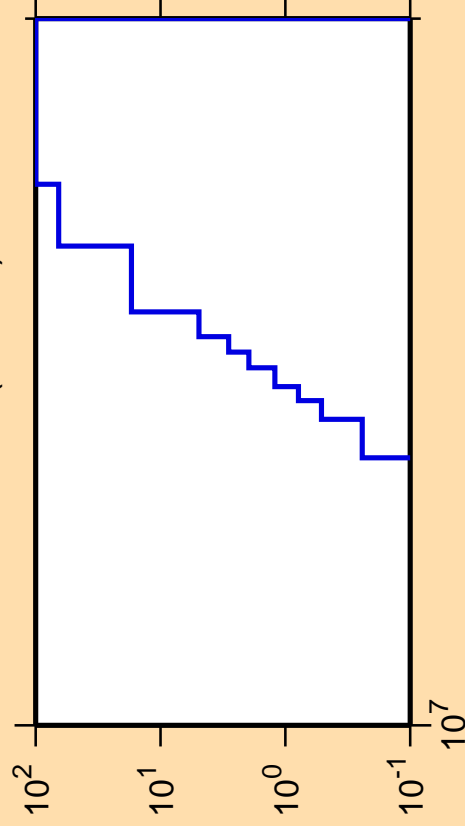
\Delta\sigma/\sigma vs. E for ^{221}\text{Ra}(\text{mt117})
