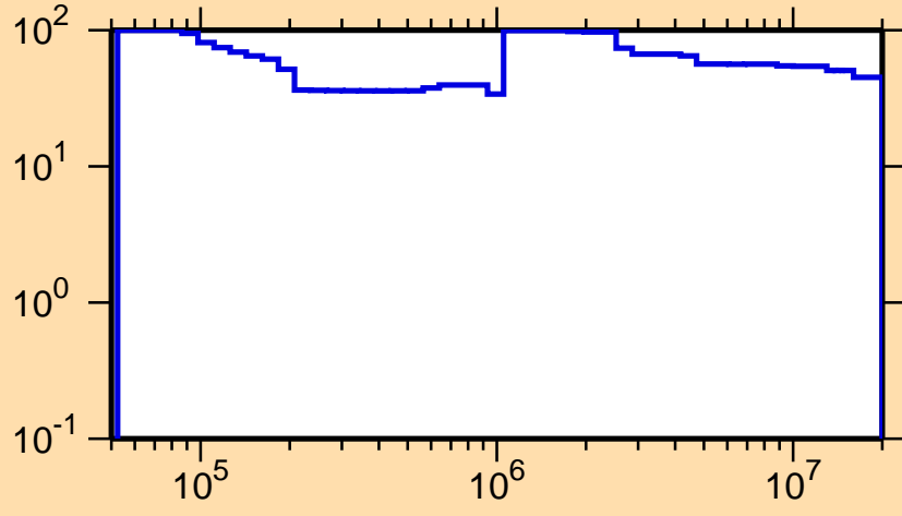
\Delta\sigma/\sigma vs. E for ^{221}\text{Ra}(n,n_1)
