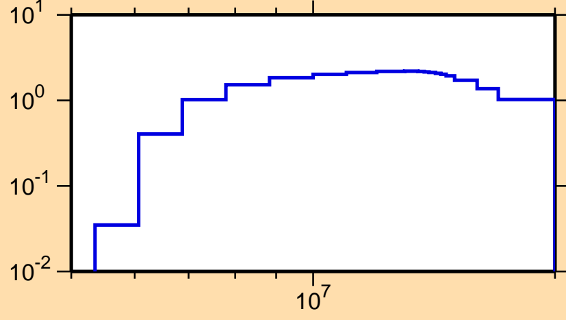
\sigma vs. E for ^{221}\text{Ra}(n,2n)
