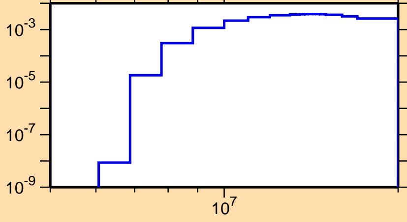
\sigma vs. E for ^{221}\text{Ra}(n,2n\alpha)
