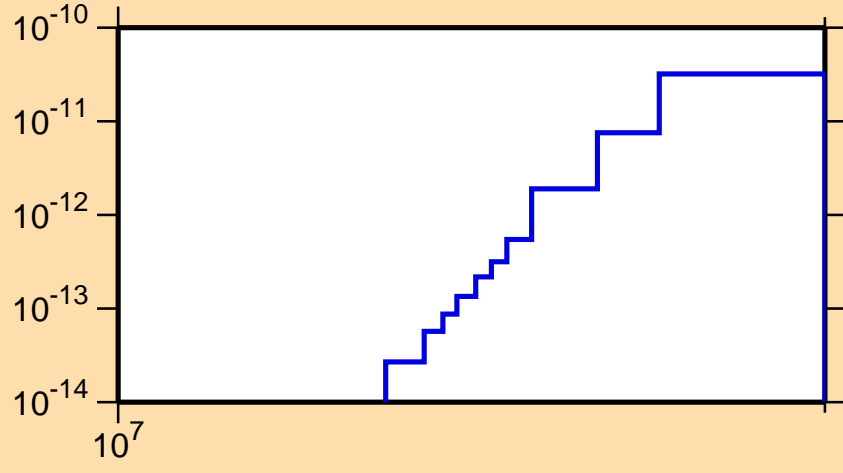
\sigma vs. E for ^{221}\text{Ra}(\text{mt117})
