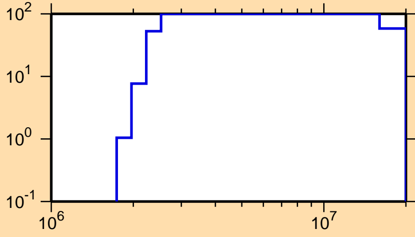
\Delta\sigma/\sigma vs. E for ^{221}\text{Ra}(n,p)
