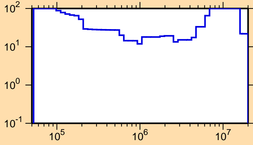
\Delta\sigma/\sigma vs. E for ^{221}\text{Ra}(n,\text{inel.})
