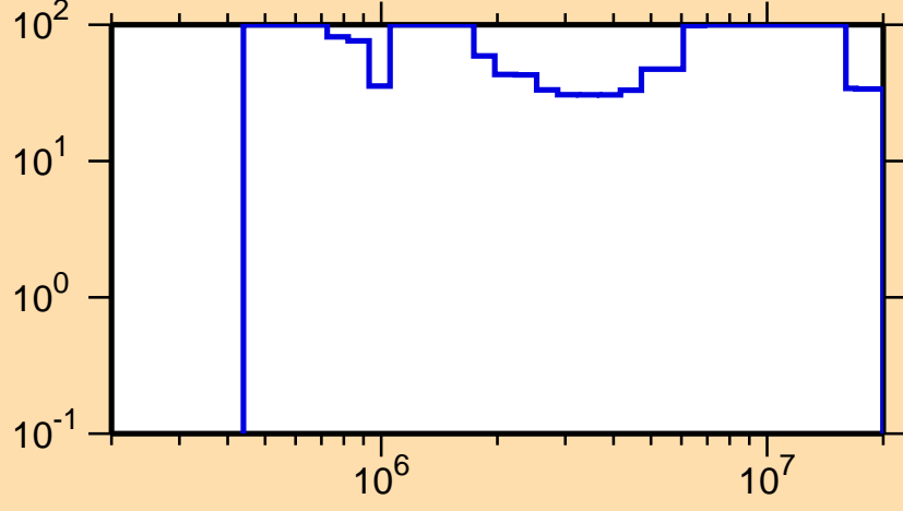
\Delta\sigma/\sigma vs. E for ^{221}\text{Ra}(n,n\text{cont.})
