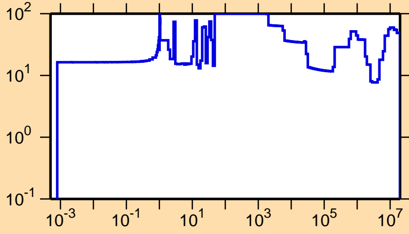
\Delta\sigma/\sigma vs. E for ^{221}\text{Ra}(n,\text{el.})
