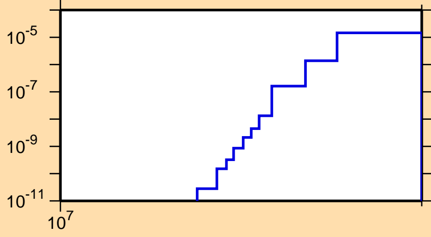
\sigma vs. E for ^{221}\text{Ra}(n,\text{nd})
