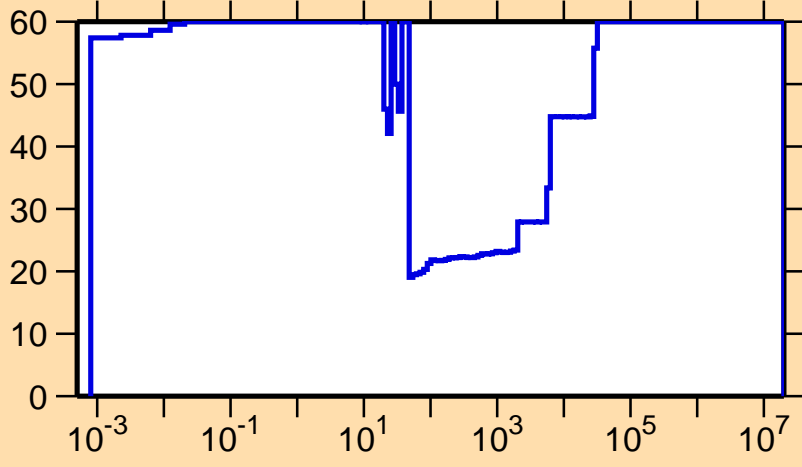
\Delta\sigma/\sigma vs. E for ^{221}\text{Ra}(n,\gamma)
