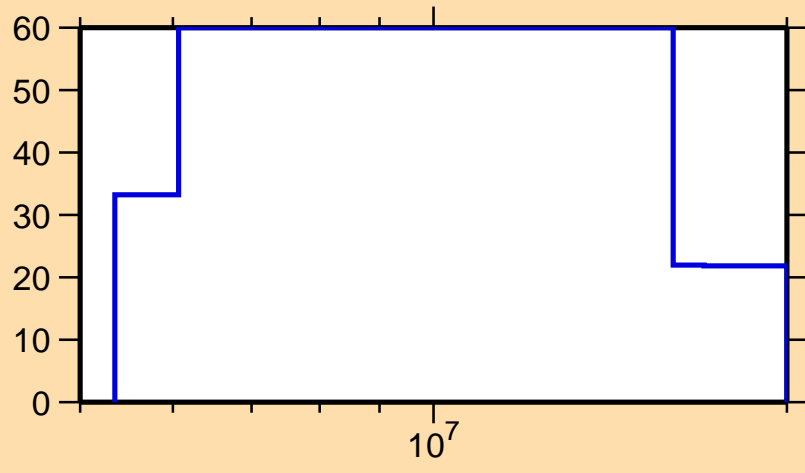
\Delta\sigma/\sigma vs. E for ^{221}\text{Ra}(n,\text{inel.})
