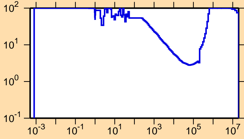
\Delta\sigma/\sigma vs. E for ^{221}\text{Ra}(n,f)
