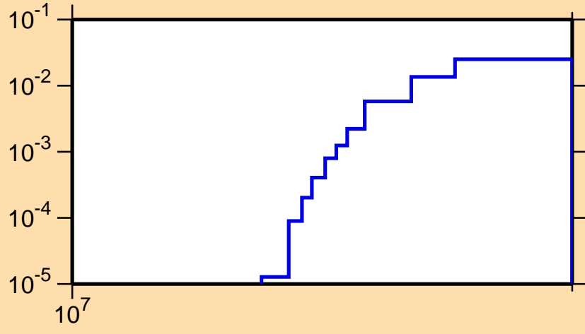
\sigma vs. E for ^{221}\text{Ra}(n,3n\alpha)
