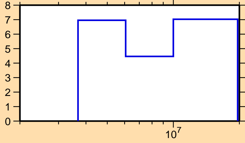
\Delta\sigma/\sigma vs. E for ^{221}\text{Ra}(n,\text{nonel.})
