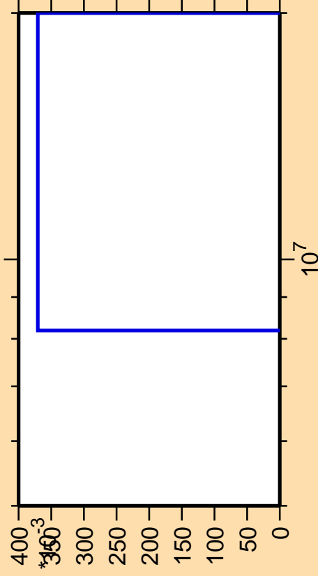
\Delta\sigma/\sigma vs. E for ^{221}\text{Ra} (mt 45)
