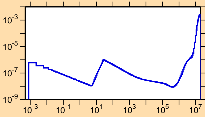
\sigma vs. E for ^{222}\text{Ra}(n,\alpha)
