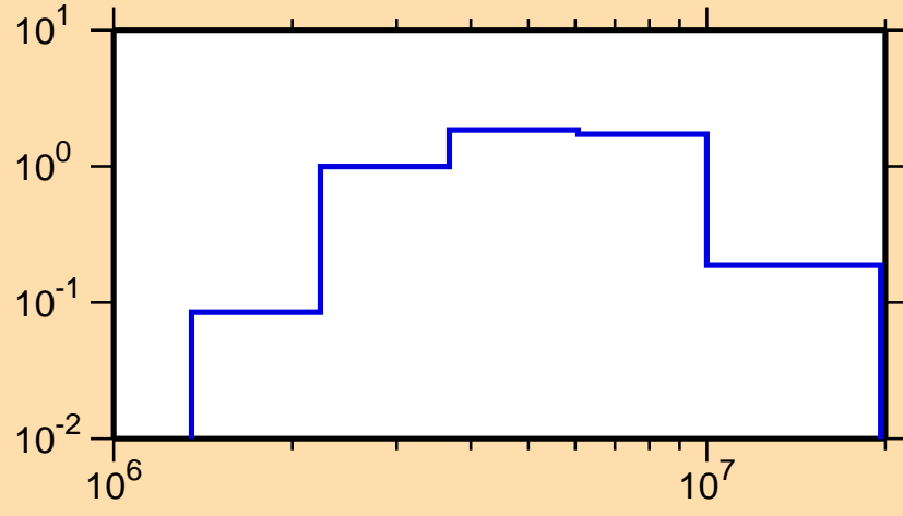
\sigma vs. E for ^{222}\text{Ra}(n,n\text{cont.})
