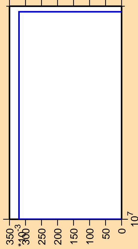
\Delta\sigma/\sigma vs. E for ^{222}\text{Ra}(\text{mt } 45)
