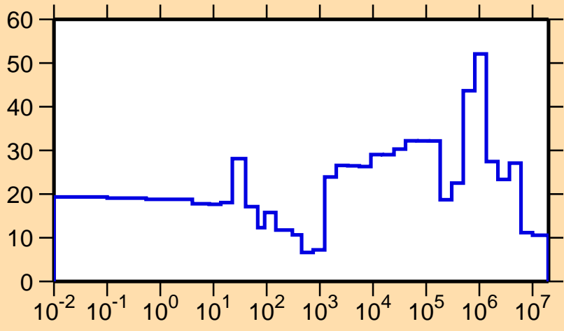
\Delta\sigma/\sigma vs. E for ^{222}\text{Ra}(n,el.)
