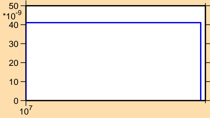
\sigma vs. E for ^{222}\text{Ra}(n,nt)
