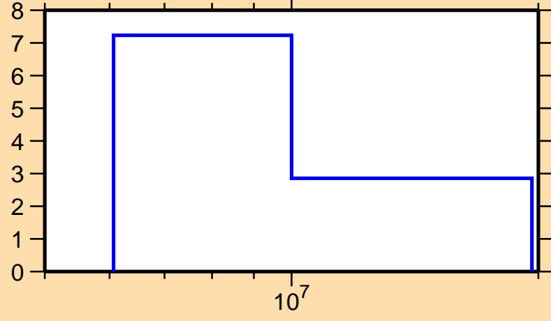
\Delta\sigma/\sigma vs. E for ^{222}\text{Ra}(n,\text{tot.})
