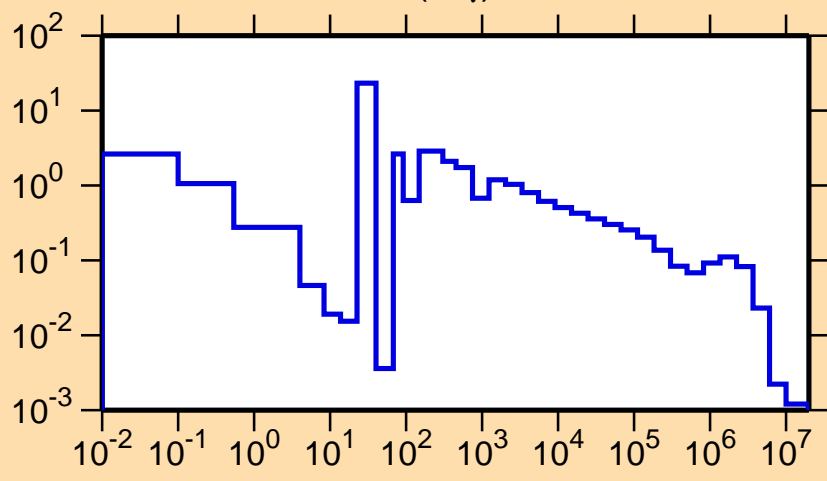
\sigma vs. E for ^{222}\text{Ra}(n,\gamma)
