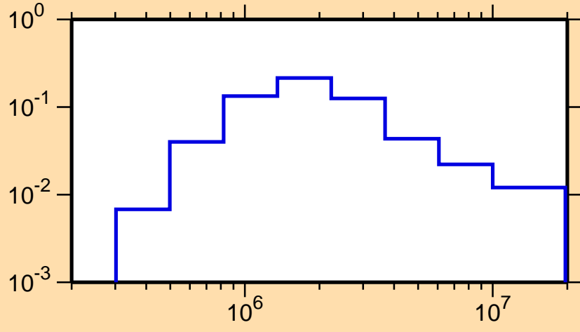
\sigma vs. E for ^{222}\text{Ra}(n,n_3)
