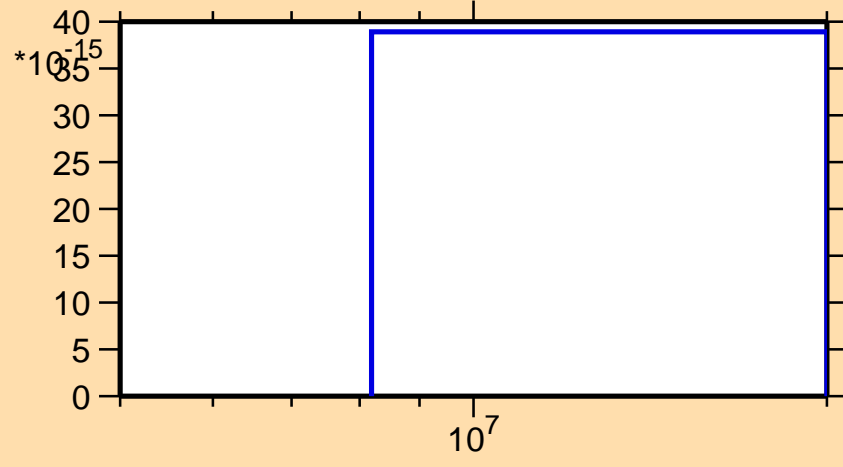
\sigma vs. E for ^{222}\text{Ra} (mt 45)
