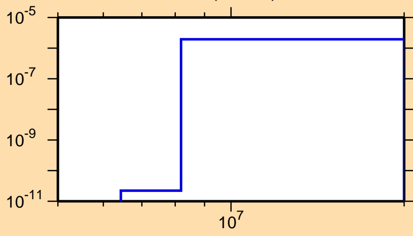
\sigma vs. E for ^{222}\text{Ra}(n,2n\alpha)
