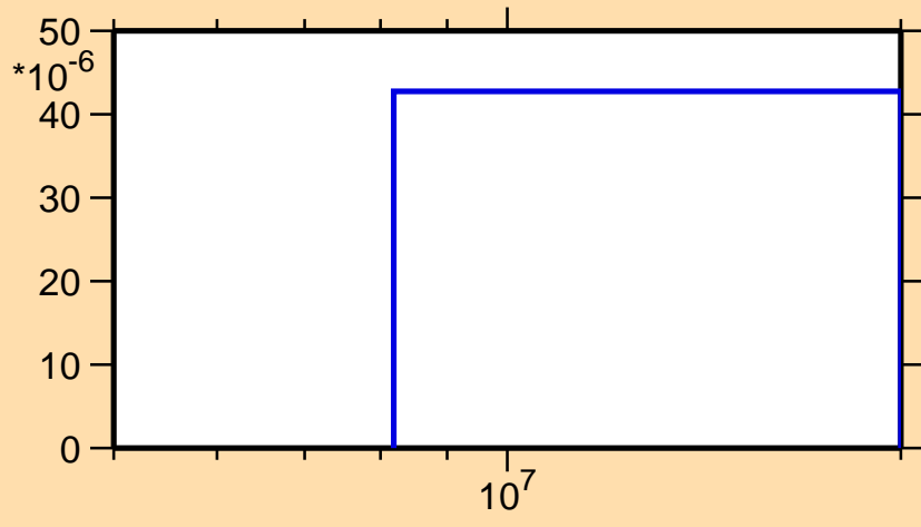
\sigma vs. E for ^{222}\text{Ra}(n,t)
