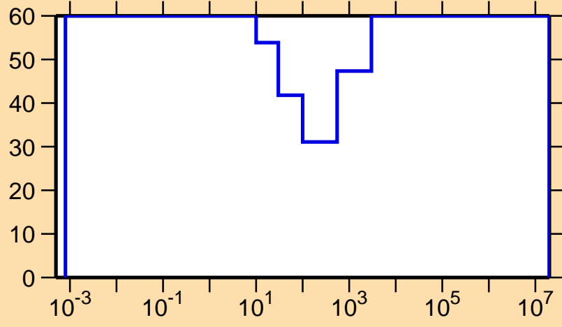
\Delta\sigma/\sigma vs. E for ^{222}\text{Ra}(n,\gamma)
