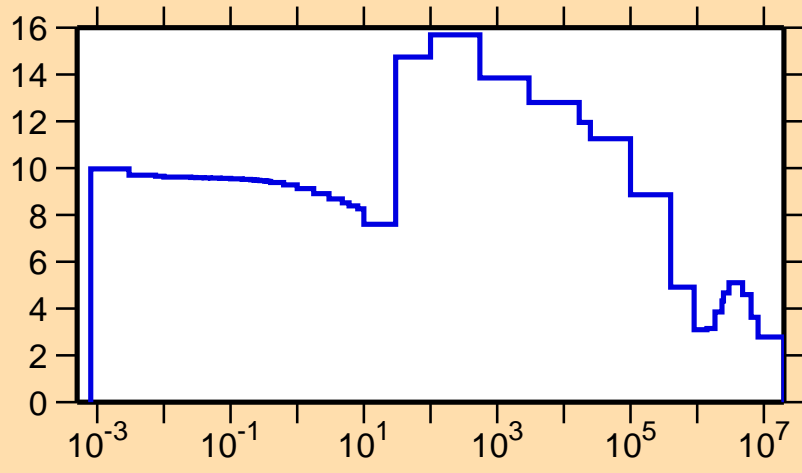
\sigma vs. E for ^{222}\text{Ra}(n,\text{el.})
