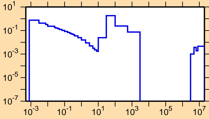
\sigma vs. E for ^{222}\text{Ra}(n,f)
