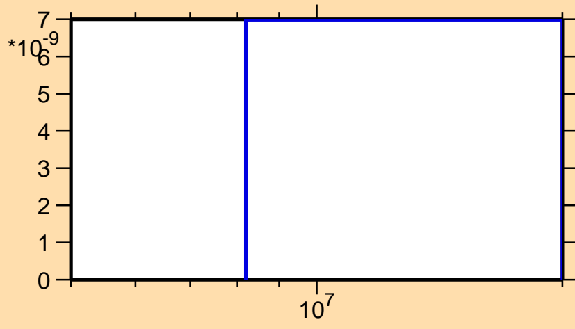
\sigma vs. E for ^{222}\text{Ra}(n,\text{nd})
