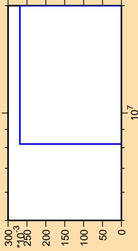
\Delta\sigma/\sigma vs. E for ^{222}\text{Ra} (mt 45)
