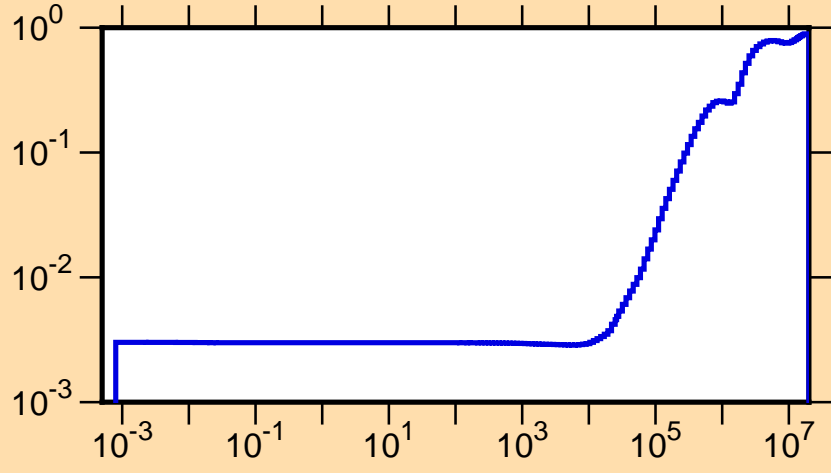
\mu vs. E for ^{223}\text{Ra}(\text{mt251})
