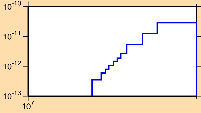
\sigma vs. E for ^{223}\text{Ra}(n,p\alpha)
