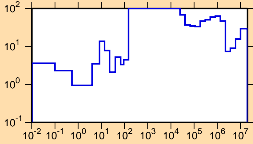
\Delta\sigma/\sigma vs. E for ^{223}\text{Ra}(n,\text{el.})
