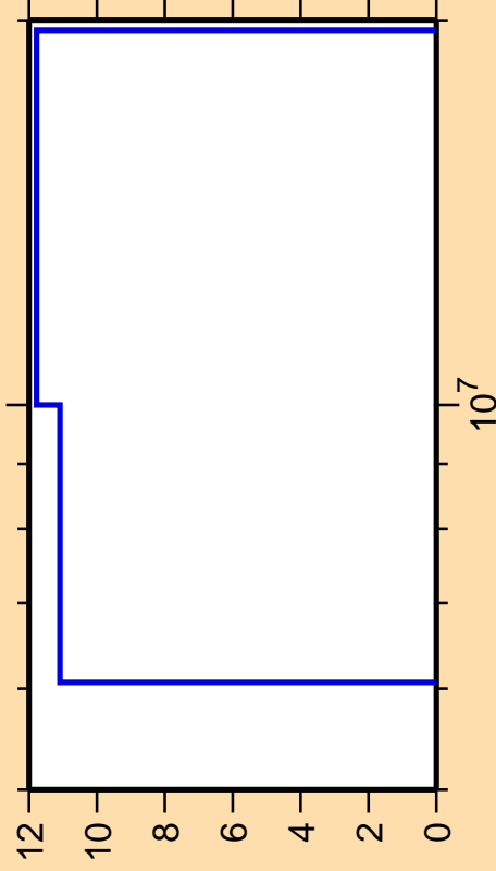
\Delta\sigma/\sigma vs. E for ^{223}\text{Ra}(n,d)
