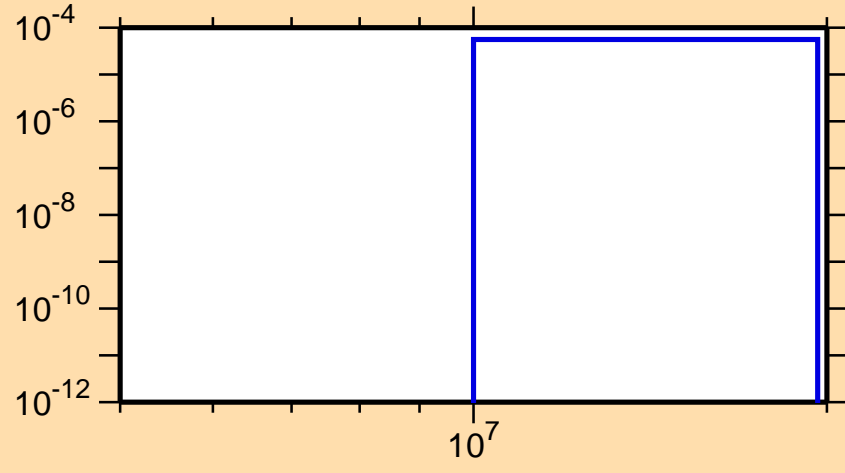
\sigma vs. E for ^{223}\text{Ra}(n,np)
