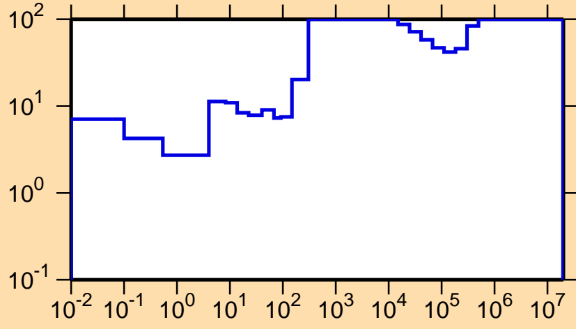
\Delta\sigma/\sigma vs. E for ^{223}\text{Ra}(n,f)
