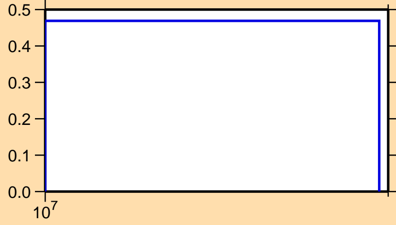
\sigma vs. E for ^{223}\text{Ra}(n,3n)
