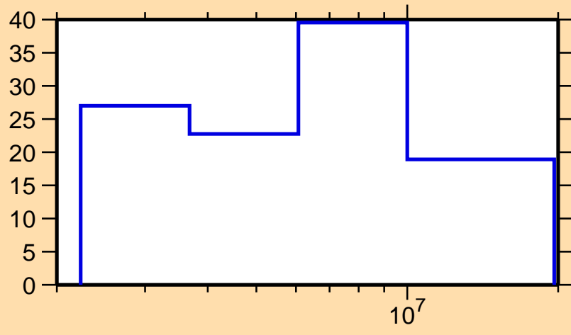
\Delta\sigma/\sigma vs. E for ^{223}\text{Ra}(n,n_1)
