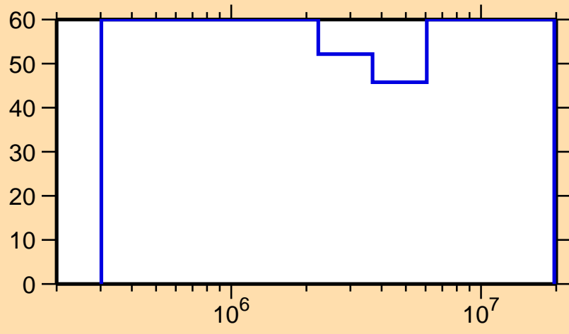
\Delta\sigma/\sigma vs. E for ^{223}\text{Ra}(n,n\text{cont.})
