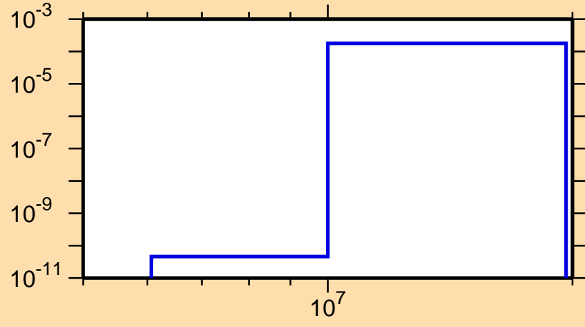
\sigma vs. E for ^{223}\text{Ra}(n,d)
