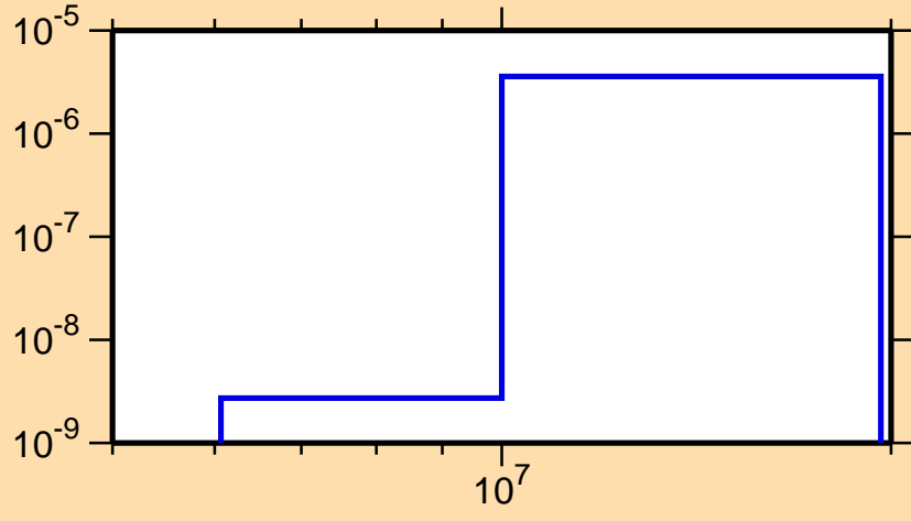
\sigma vs. E for ^{223}\text{Ra}(n,2n\alpha)
