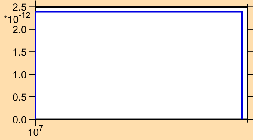
\sigma vs. E for ^{223}\text{Ra}(n,p\alpha)
