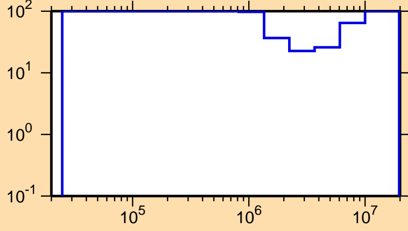
\Delta\sigma/\sigma vs. E for ^{223}\text{Ra}(n,\text{inel.})
