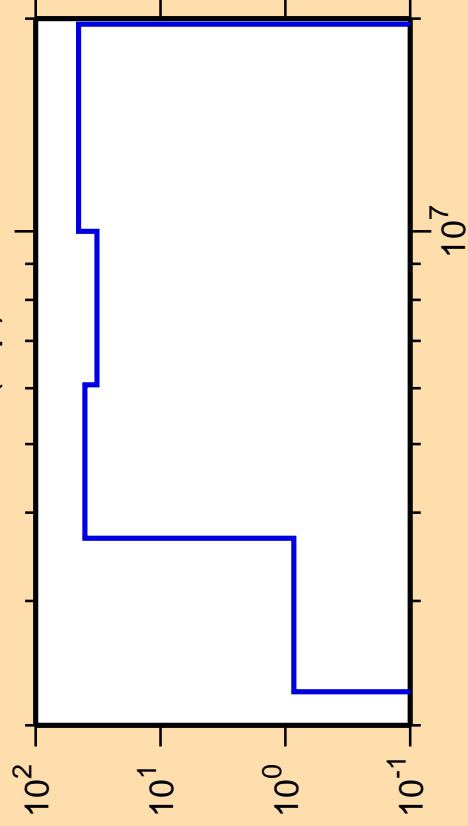
\Delta\sigma/\sigma vs. E for ^{223}\text{Ra}(n,p)
