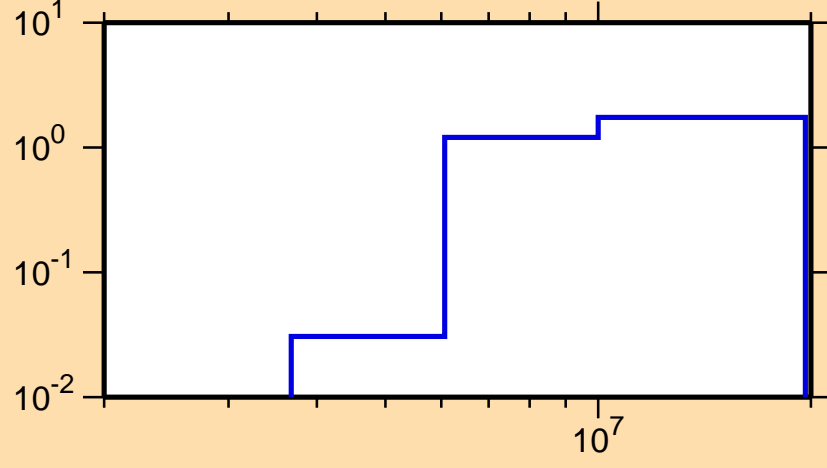
\sigma vs. E for ^{223}\text{Ra}(n,2n)
