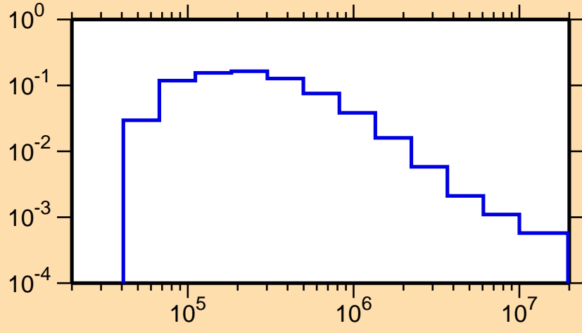
\sigma vs. E for ^{223}\text{Ra}(n,n_2)
