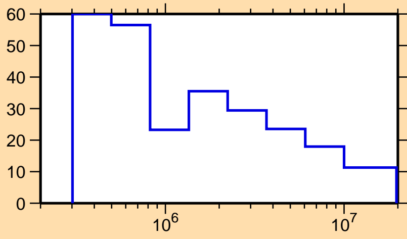
\Delta\sigma/\sigma vs. E for ^{223}\text{Ra}(n,\text{nonel.})
