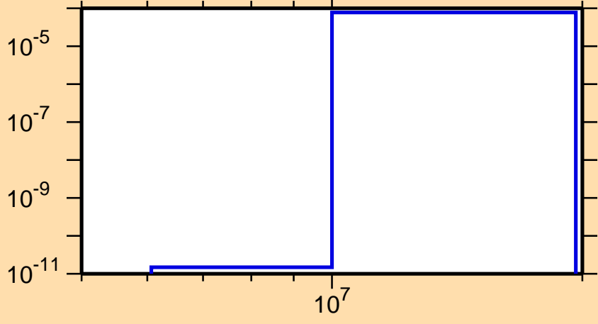
\sigma vs. E for ^{223}\text{Ra}(n,t)
