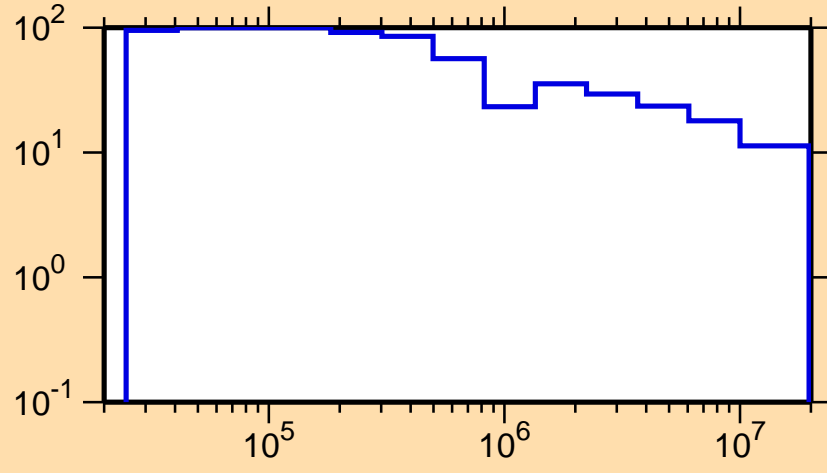
\Delta\sigma/\sigma vs. E for ^{223}\text{Ra}(n,\text{nonel.})
