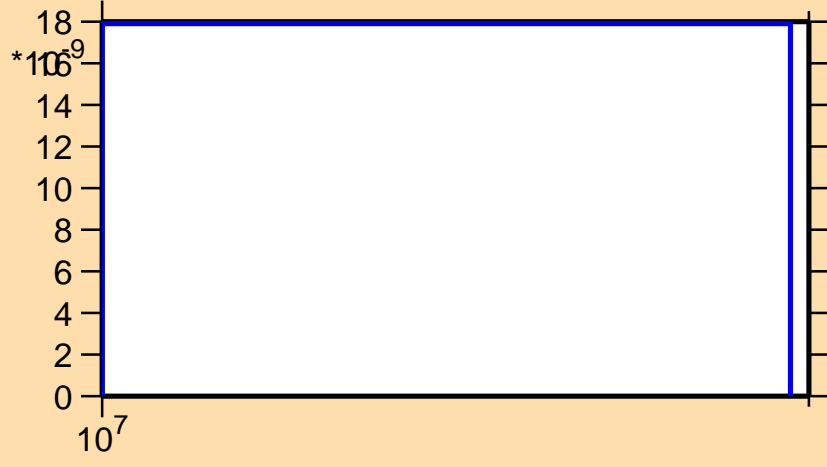
\sigma vs. E for ^{223}\text{Ra}(n,2np)
