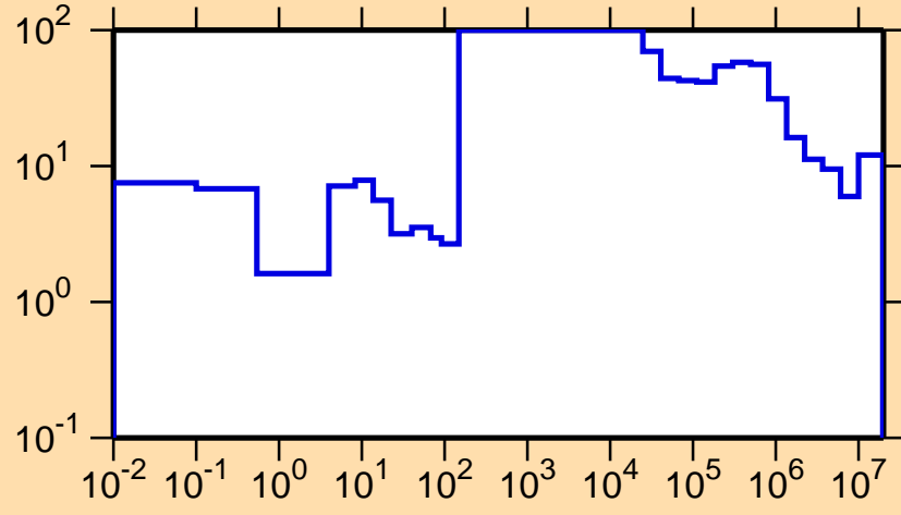
\Delta\sigma/\sigma vs. E for ^{223}\text{Ra}(n,\text{tot.})
