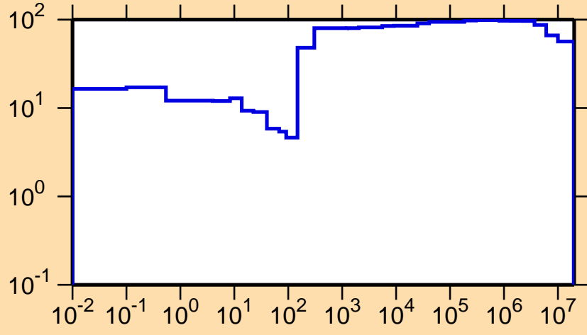
\Delta\sigma/\sigma vs. E for ^{223}\text{Ra}(n,\gamma)
