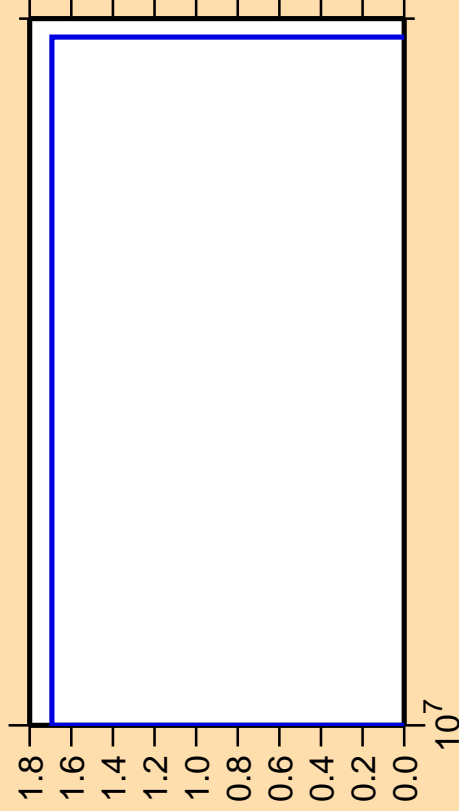
\Delta\sigma/\sigma vs. E for ^{223}\text{Ra}(n,\text{He3})
