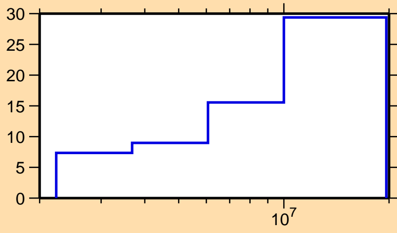
\Delta\sigma/\sigma vs. E for ^{223}\text{Ra}(n,\text{el.})
