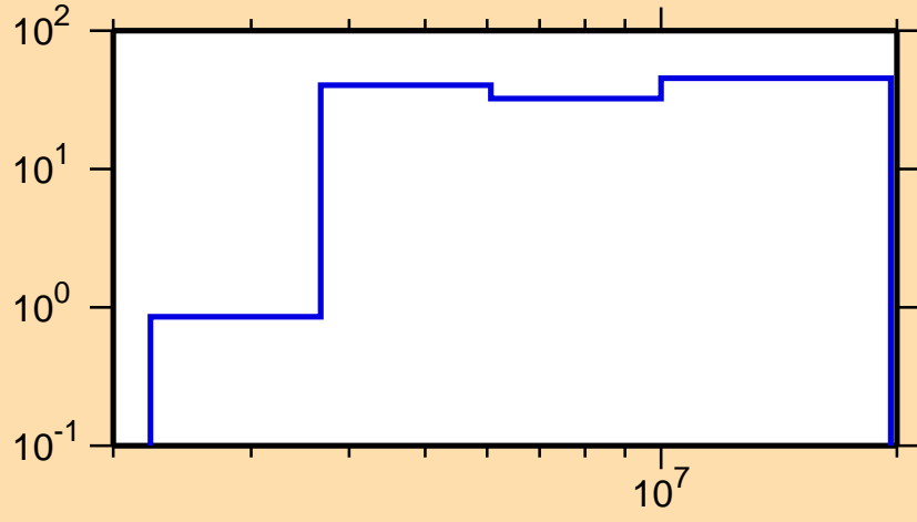
\Delta\sigma/\sigma vs. E for ^{223}\text{Ra}(n,p)
