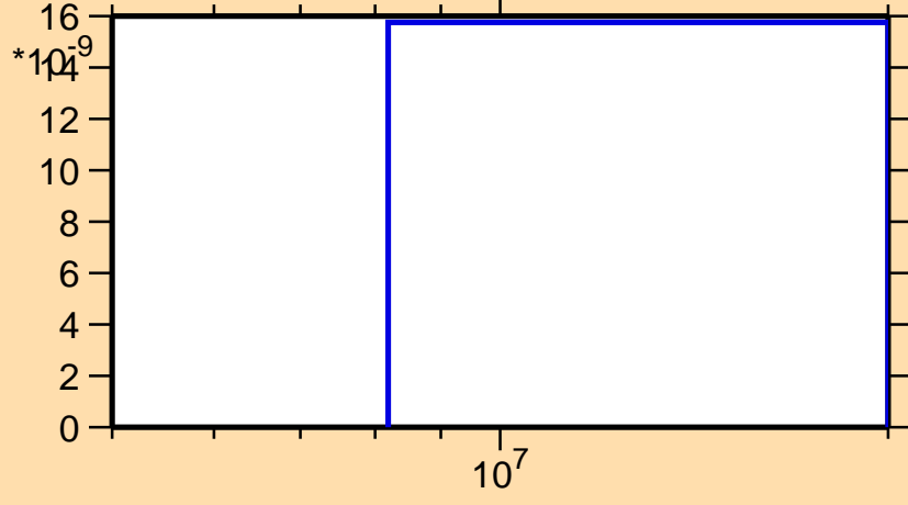
\sigma vs. E for ^{223}\text{Ra}(n,2np)
