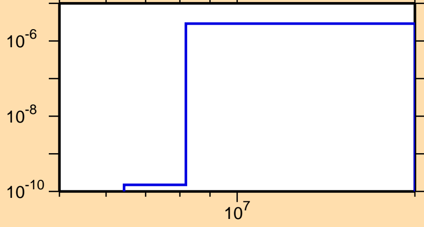
\sigma vs. E for ^{223}\text{Ra}(n,2n\alpha)
