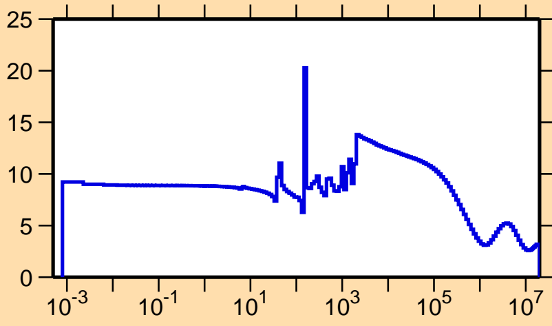
\sigma vs. E for ^{224}\text{Ra}(n,\text{el.})
