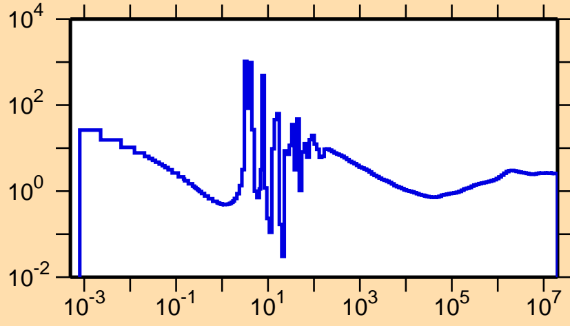
\sigma vs. E for ^{225}\text{Ra}(n,\text{nonel.})
