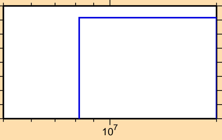
\sigma vs. E for ^{225}\text{Ra}(n,\text{nd})
