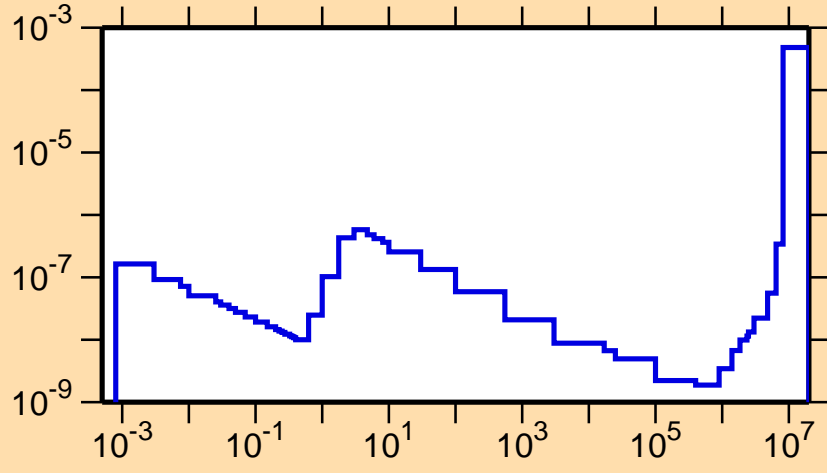
\sigma vs. E for ^{225}\text{Ra}(n,\alpha)
