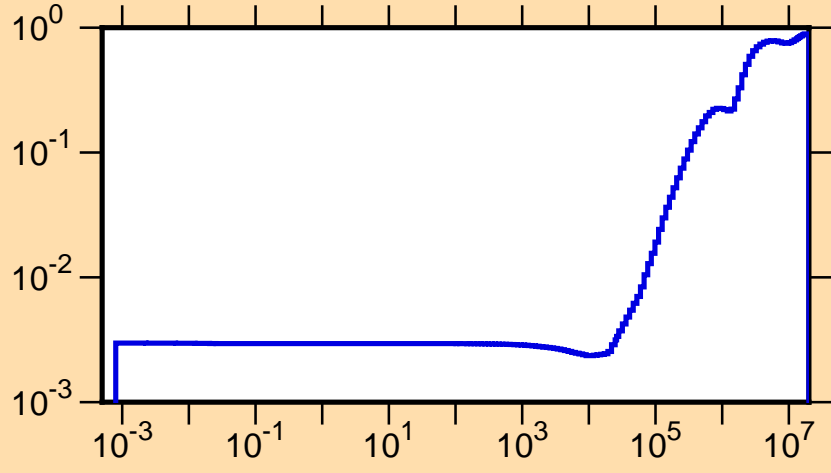
\mu vs. E for ^{226}\text{Ra}(\text{mt251})
