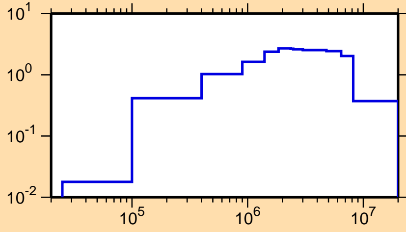
\sigma vs. E for ^{226}\text{Ra}(n,\text{inel.})
