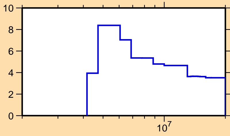
\Delta\sigma/\sigma vs. E for ^{227}\text{Ra}(n,\text{nonel.})
