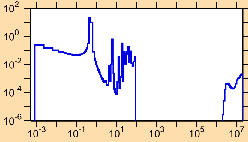
\sigma vs. E for ^{227}\text{Ra}(n,f)
