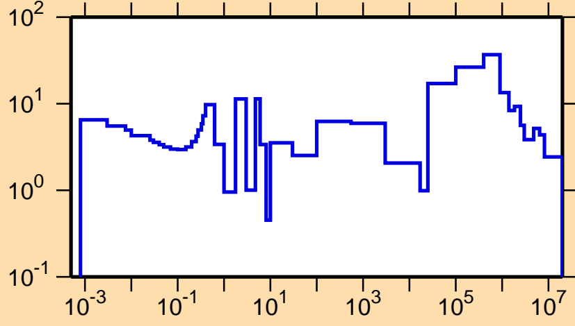
\Delta\sigma/\sigma vs. E for ^{227}\text{Ra}(n,tot.)
