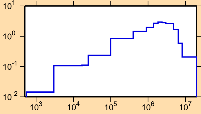
\sigma vs. E for ^{227}\text{Ra}(n,\text{inel.})
