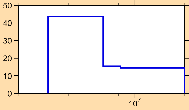
\Delta\sigma/\sigma vs. E for ^{227}\text{Ra}(n,2n)
