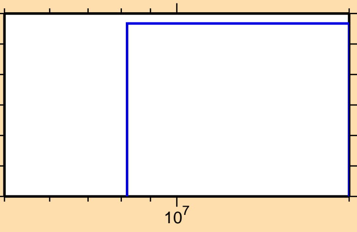
\sigma vs. E for ^{227}\text{Ra} (mt 42)
