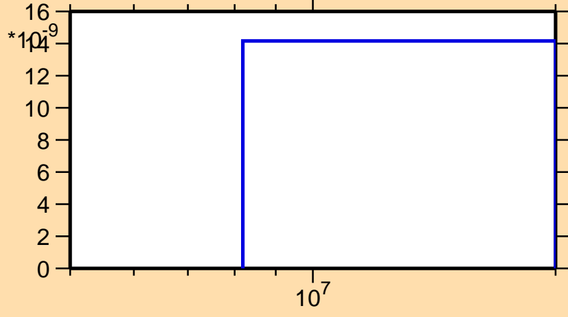
\sigma vs. E for ^{227}\text{Ra}(n,nt)
