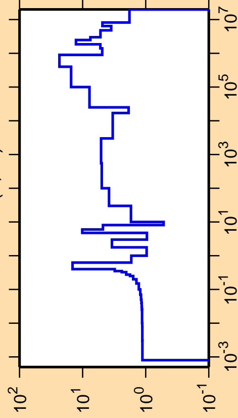
\Delta\sigma/\sigma vs. E for ^{227}\text{Ra}(n,\text{el.})
