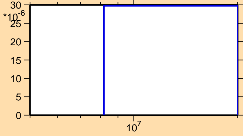
\sigma vs. E for ^{227}\text{Ra}(n,d)
