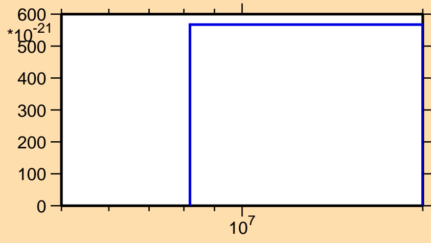
\sigma vs. E for ^{227}\text{Ra} (mt 42)
