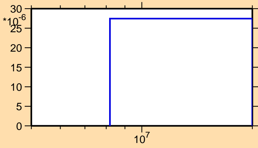
\sigma vs. E for ^{227}\text{Ra}(n,t)
