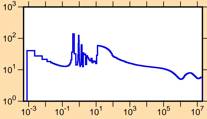
\sigma vs. E for ^{229}\text{Ra}(n,\text{tot.})
