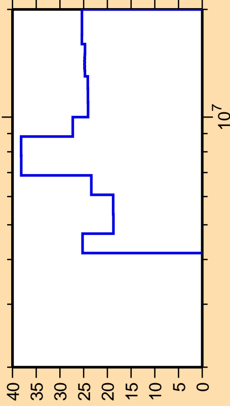
\Delta\sigma/\sigma vs. E for ^{229}\text{Ra}(n,n\text{cont.})
