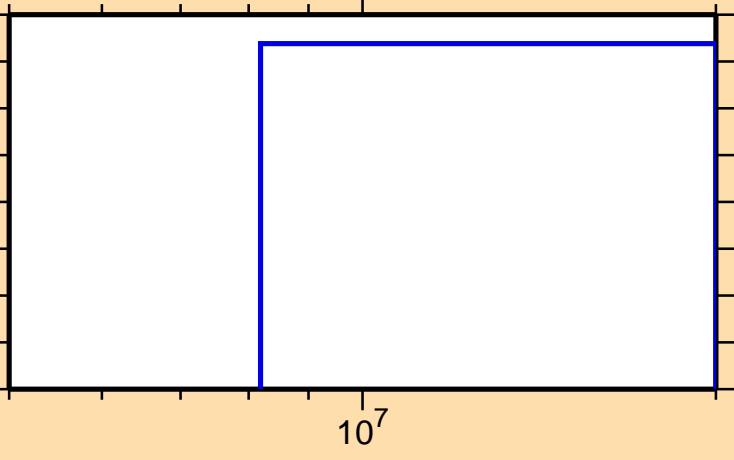
\sigma vs. E for ^{229}\text{Ra}(n,d)
