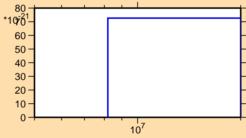
\sigma vs. E for ^{229}\text{Ra} (mt 42)
