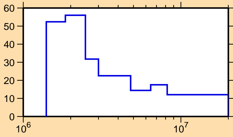
\Delta\sigma/\sigma vs. E for ^{229}\text{Ra}(n,n\text{onel.})
