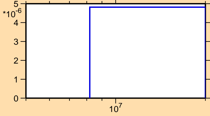
\sigma vs. E for ^{230}\text{Ra}(n,d)
