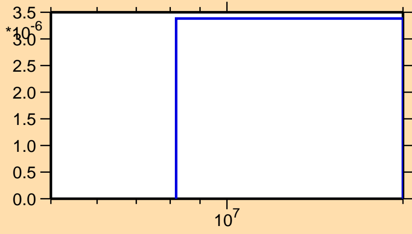
\sigma vs. E for ^{230}\text{Ra}(n,t)
