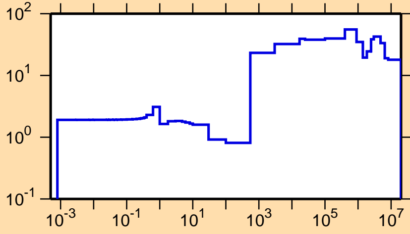
\Delta\sigma/\sigma vs. E for ^{230}\text{Ra}(n,el.)
