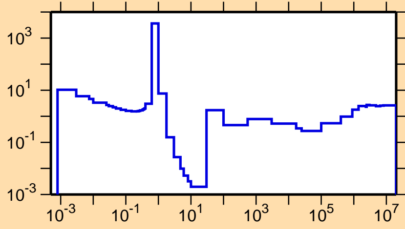
\sigma vs. E for ^{230}\text{Ra}(n,\text{nonel.})
