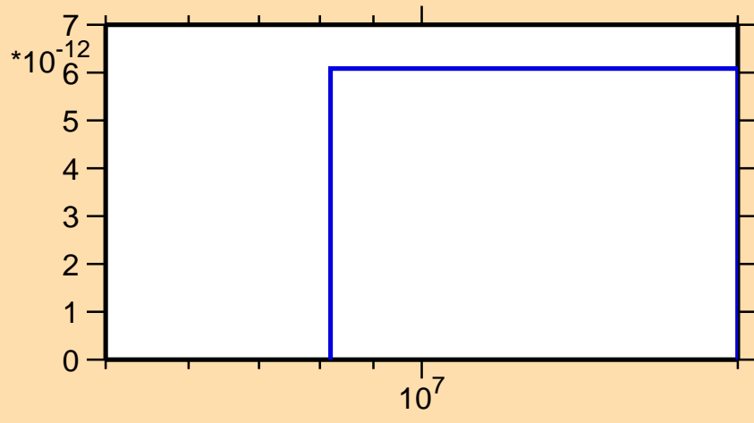
\sigma vs. E for ^{230}\text{Ra}(n,2np)
