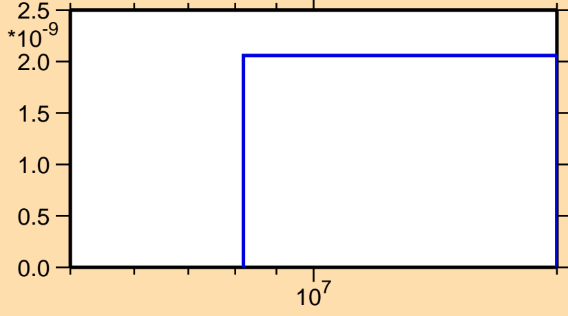
\sigma vs. E for ^{230}\text{Ra}(n,nt)
