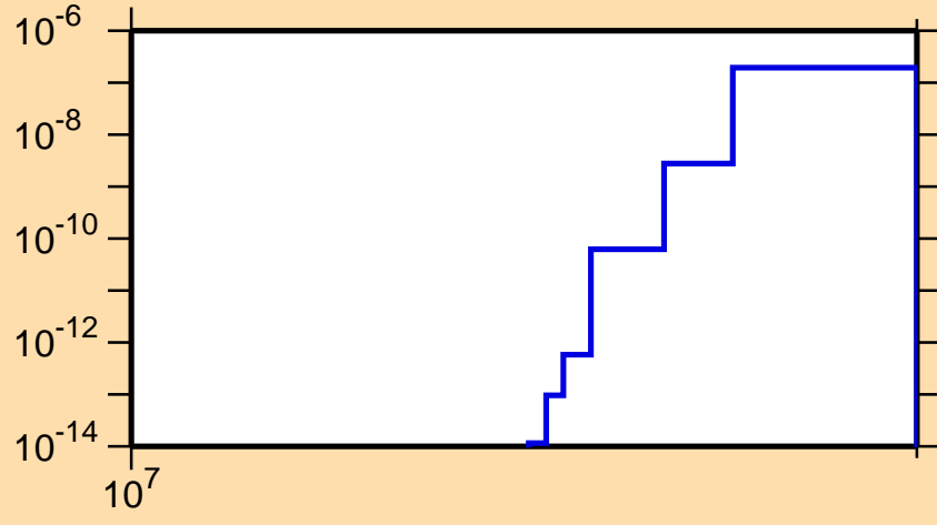
\sigma vs. E for ^{231}\text{Ra}(n,\text{nd})
