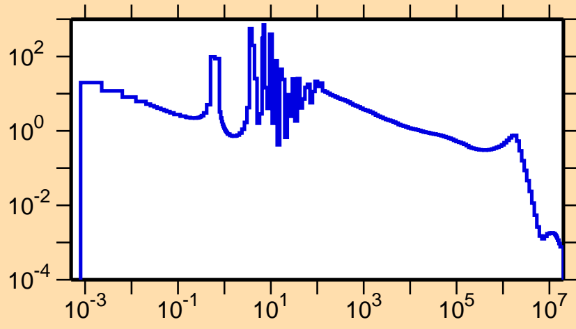
\sigma vs. E for ^{231}\text{Ra}(n,\gamma)
