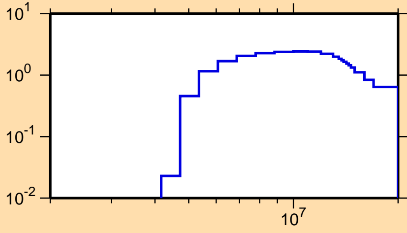
\sigma vs. E for ^{231}\text{Ra}(n,2n)
