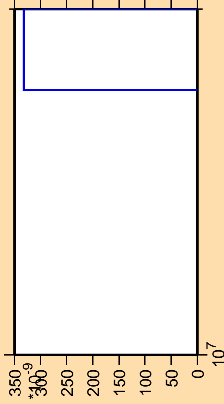
\Delta\sigma/\sigma vs. E for ^{231}\text{Ra} (mt 42)
