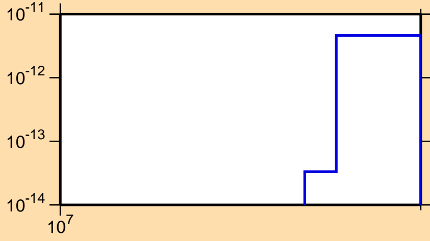
\sigma vs. E for ^{231}\text{Ra}(n,3n\alpha)
