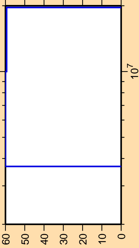
\Delta\sigma/\sigma vs. E for ^{231}\text{Ra}(n,n\text{cont.})
