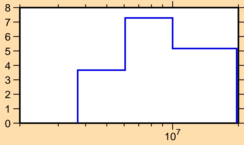
\Delta\sigma/\sigma vs. E for ^{231}\text{Ra}(n,\text{tot.})
