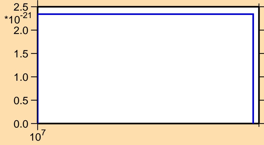
\sigma vs. E for ^{231}\text{Ra} (mt 42)
