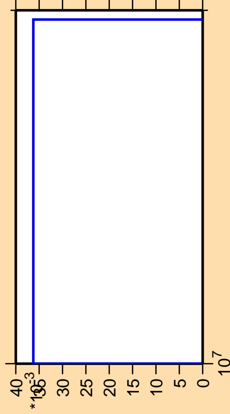
\Delta\sigma/\sigma vs. E for ^{231}\text{Ra}(n,3n\alpha)
