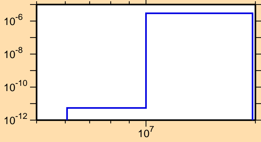
\sigma vs. E for ^{231}\text{Ra}(n,n\alpha)
