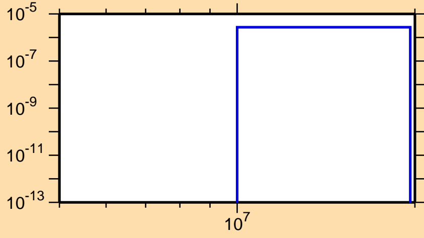
\sigma vs. E for ^{231}\text{Ra}(n,np)
