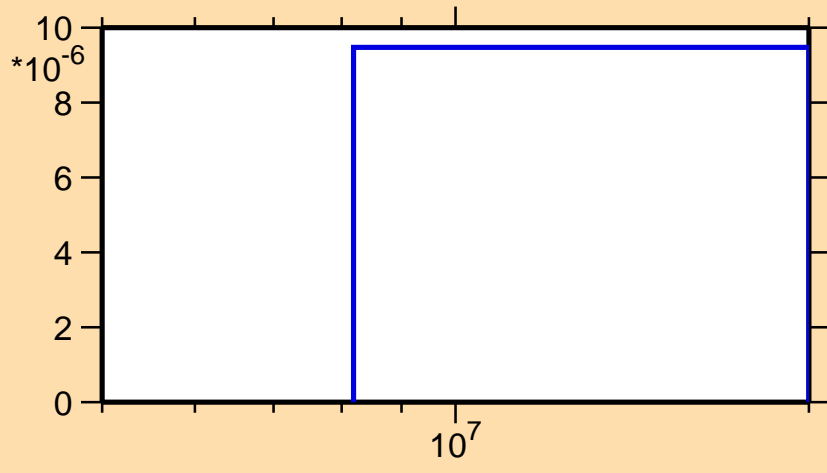
\sigma vs. E for ^{231}\text{Ra}(n,t)
