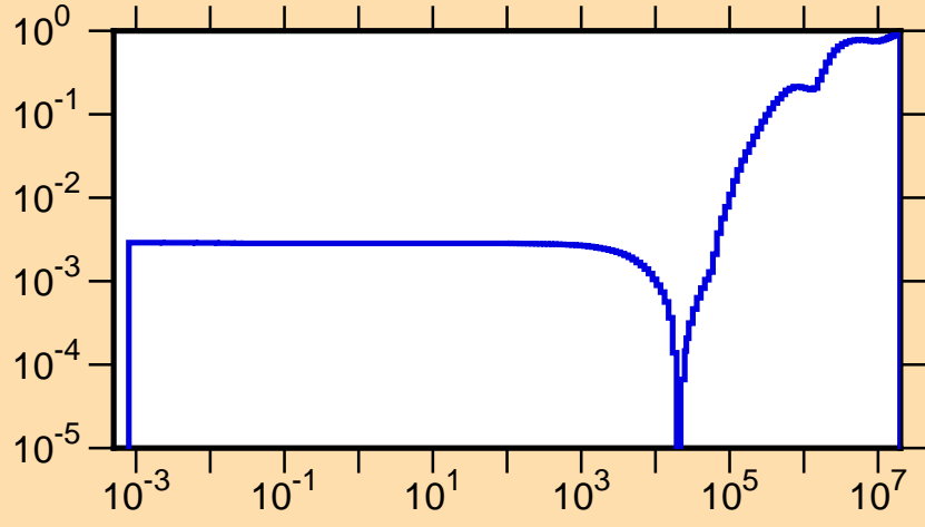
\mu vs. E for ^{232}\text{Ra}(\text{mt251})
