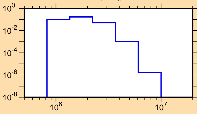
\sigma vs. E for ^{232}\text{Ra}(n,n_4)
