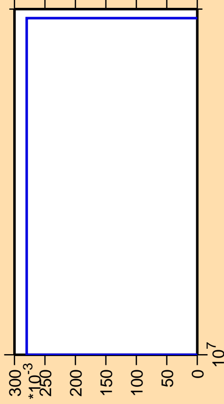
\Delta\sigma/\sigma vs. E for ^{232}\text{Ra}(n,3n\alpha)
