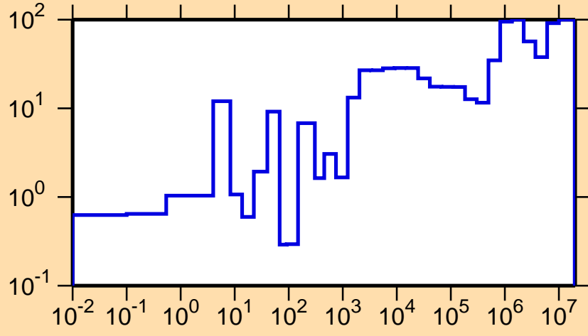
\Delta\sigma/\sigma vs. E for ^{232}\text{Ra}(n,el.)
