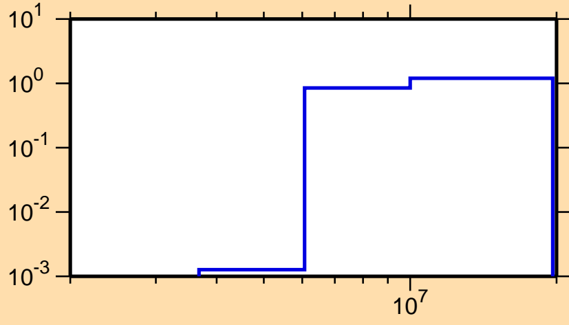
\sigma vs. E for ^{232}\text{Ra}(n,2n)
