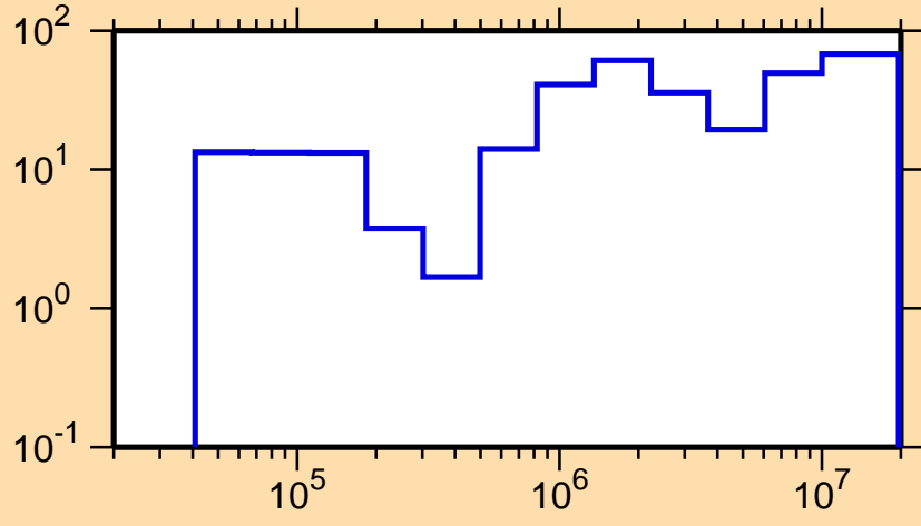
\Delta\sigma/\sigma vs. E for ^{2332}\text{Ra}(n,\text{tot.})
