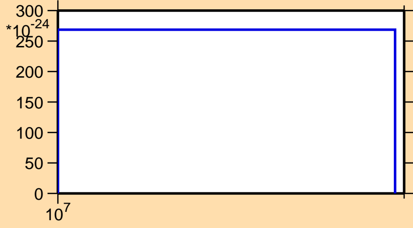
\sigma vs. E for ^{232}\text{Ra}(\text{mt } 42)
