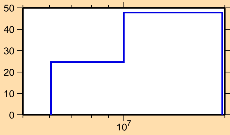
\Delta\sigma/\sigma vs. E for ^{232}\text{Ra}(n,p)
