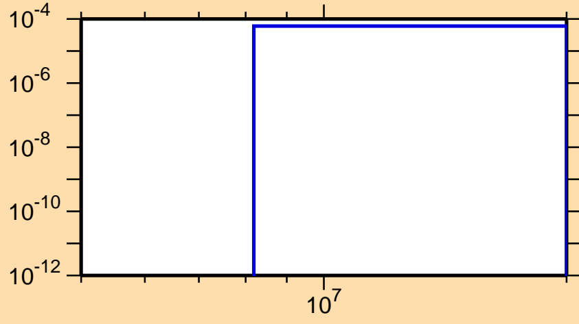
\sigma vs. E for ^{232}\text{Ra}(n,p)
