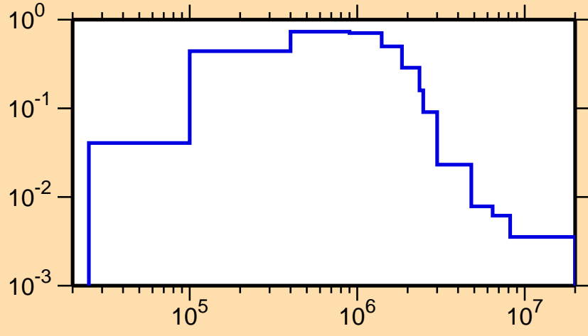
\sigma vs. E for ^{232}\text{Ra}(n,n_1)
