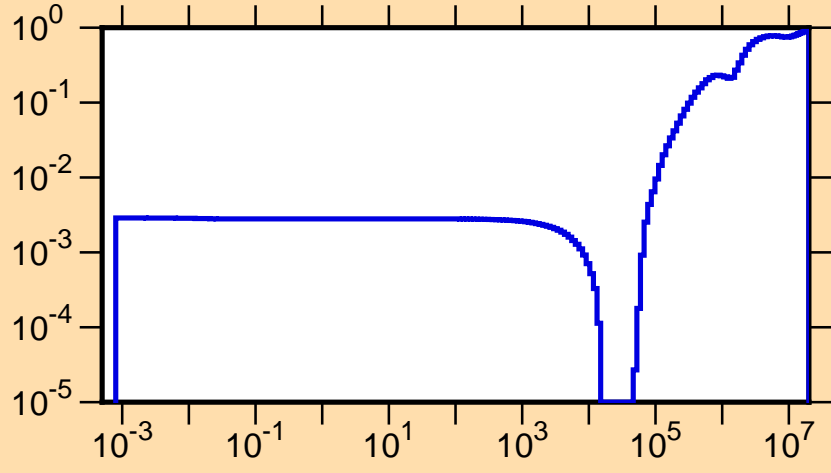
\mu vs. E for ^{233}\text{Ra}(\text{mt251})
