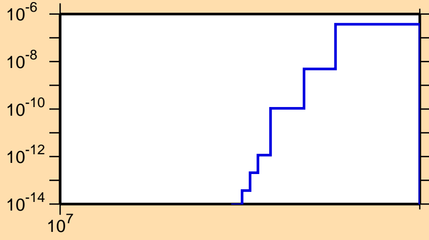
\sigma vs. E for ^{233}\text{Ra}(n,nt)
