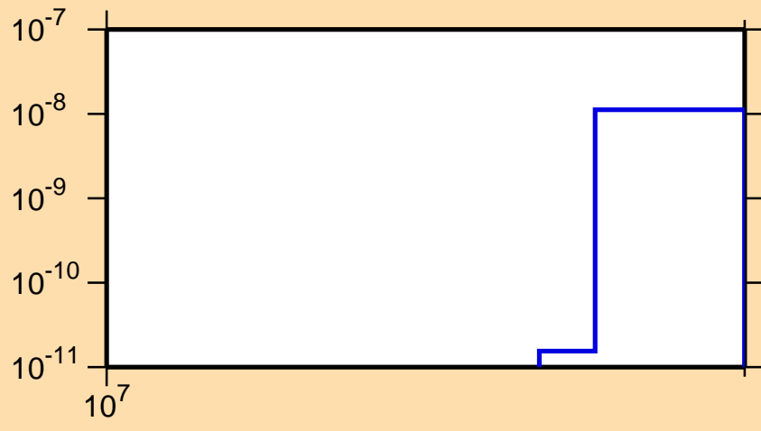
\sigma vs. E for ^{233}\text{Ra}(n,2np)
