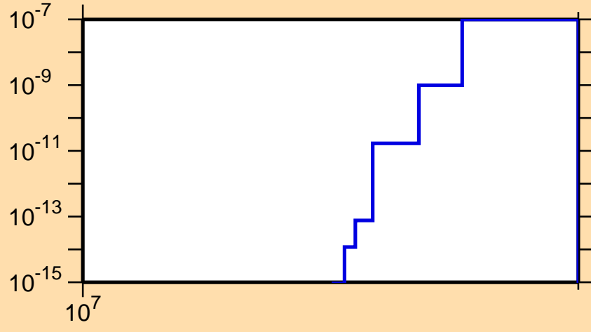
\sigma vs. E for ^{233}\text{Ra}(n,\text{nd})
