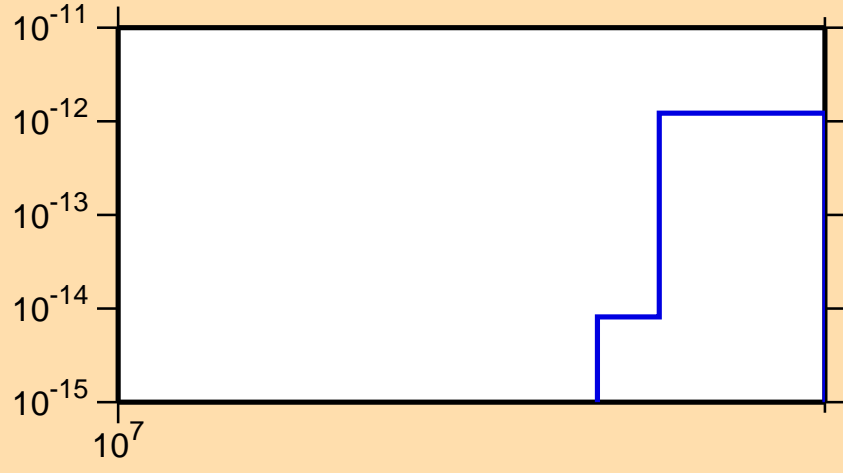
\sigma vs. E for ^{233}\text{Ra}(n,3n\alpha)
