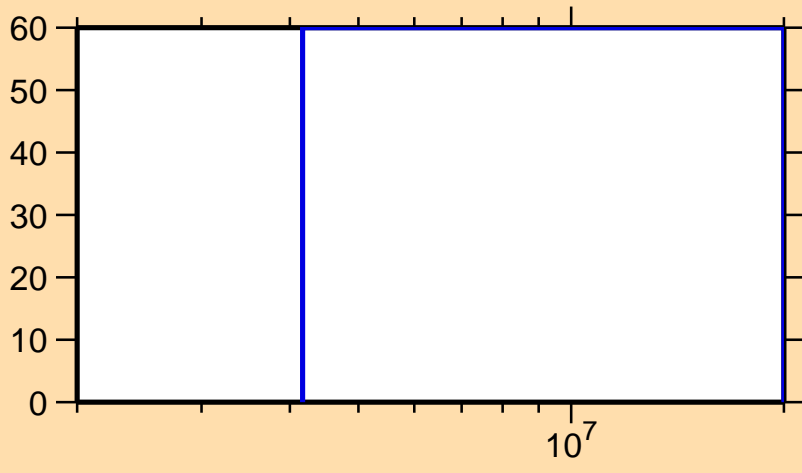
\Delta\sigma/\sigma vs. E for ^{233}\text{Ra}(n,2n)
