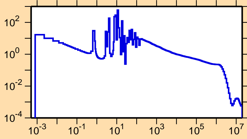
\sigma vs. E for ^{233}\text{Ra}(n,\gamma)
