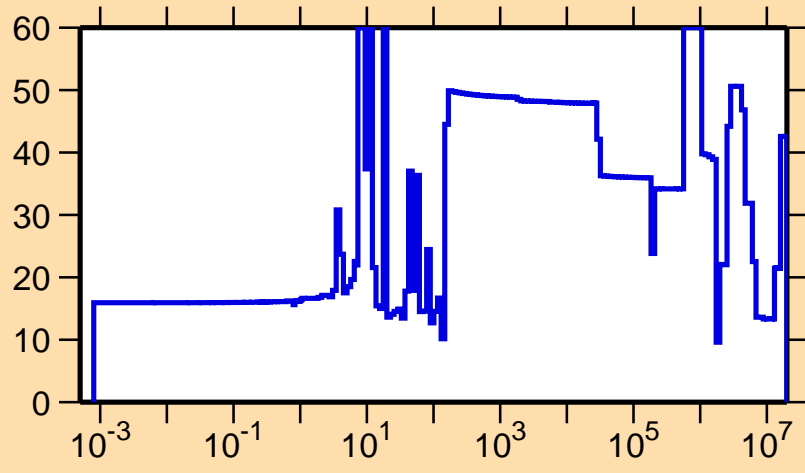
\Delta\sigma/\sigma vs. E for ^{233}\text{Ra}(n,el.)
