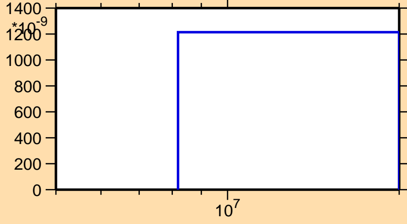
\sigma vs. E for ^{233}\text{Ra}(n,n\alpha)
