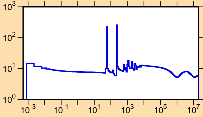
\sigma vs. E for ^{234}\text{Ra}(n,\text{tot.})
