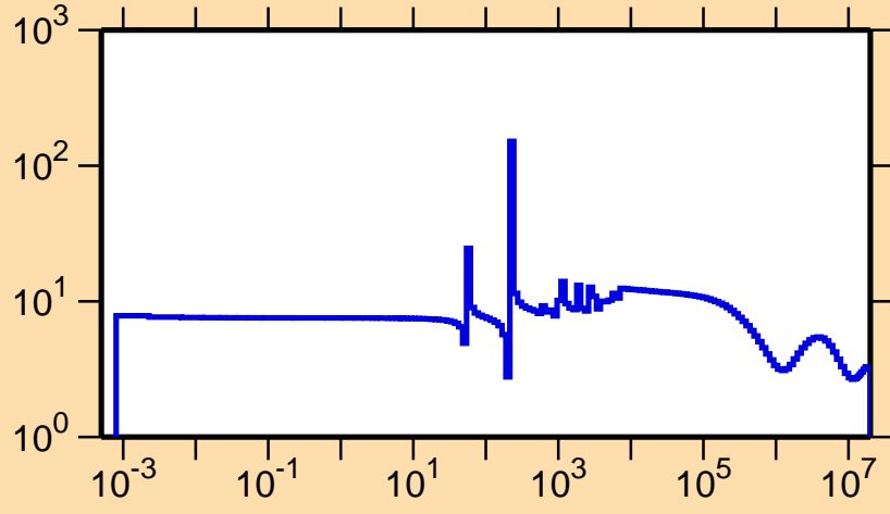
\sigma vs. E for ^{234}\text{Ra}(n,\text{el.})
