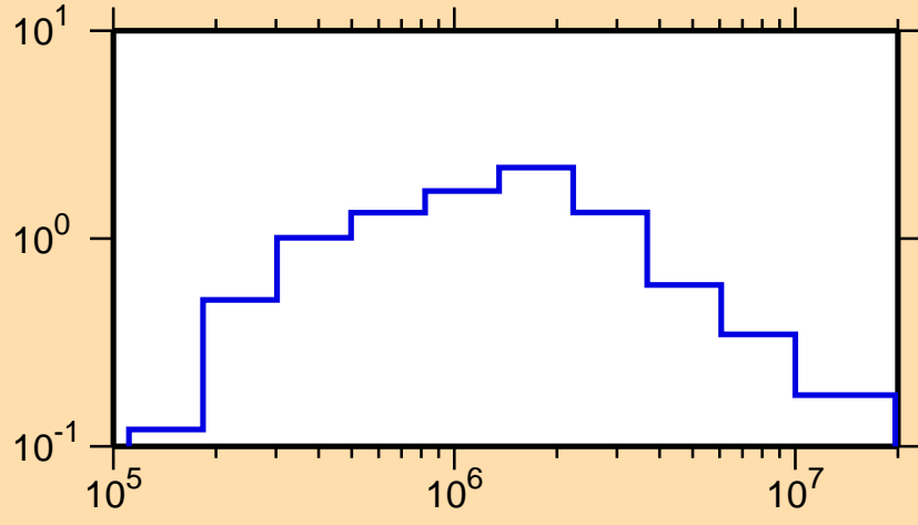
\sigma vs. E for ^{234}\text{Ra}(n,n_1)
