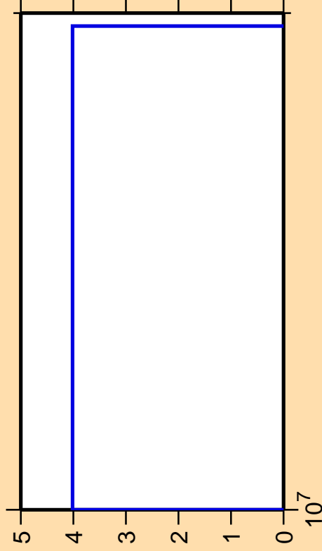
\Delta\sigma/\sigma vs. E for ^{234}\text{Ra}(n,2np)
