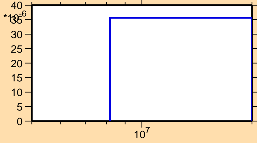
\sigma vs. E for ^{234}\text{Ra}(n,p)
