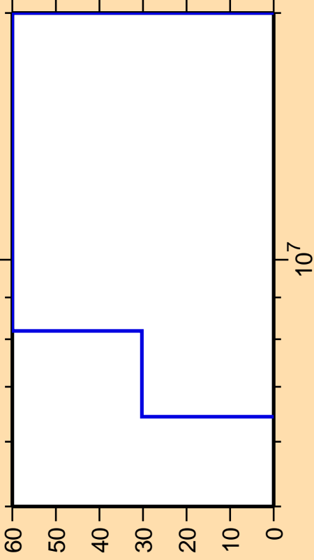
\Delta\sigma/\sigma vs. E for ^{234}\text{Ra}(n,\alpha)
