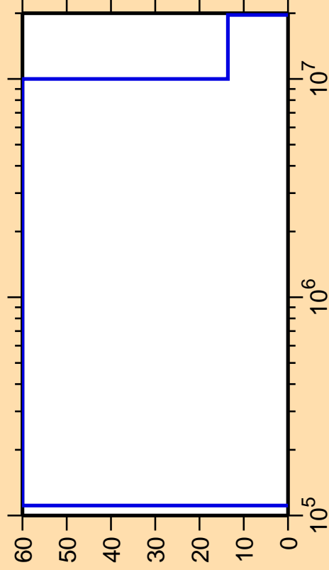
\Delta\sigma/\sigma vs. E for ^{235}\text{Ra}(n,\gamma)
