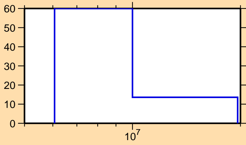
\Delta\sigma/\sigma vs. E for ^{235}\text{Ra}(n,\gamma)
