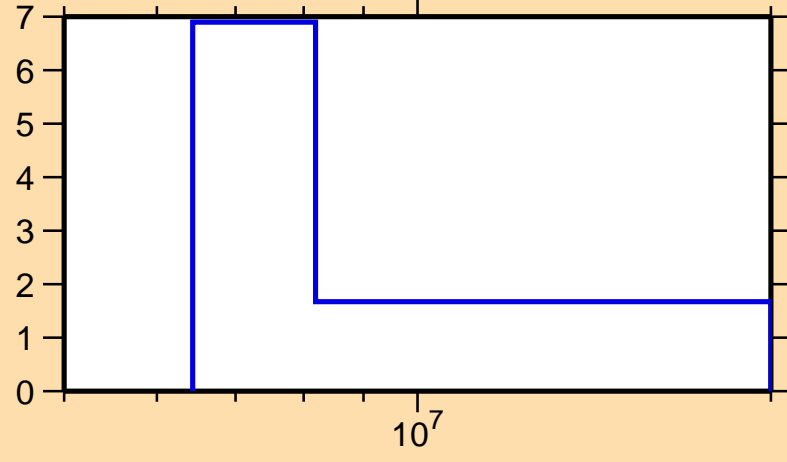
\Delta\sigma/\sigma vs. E for ^{235}\text{Ra}(n,\text{nonel.})
