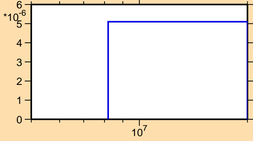
\sigma vs. E for ^{235}\text{Ra}(n,t)
