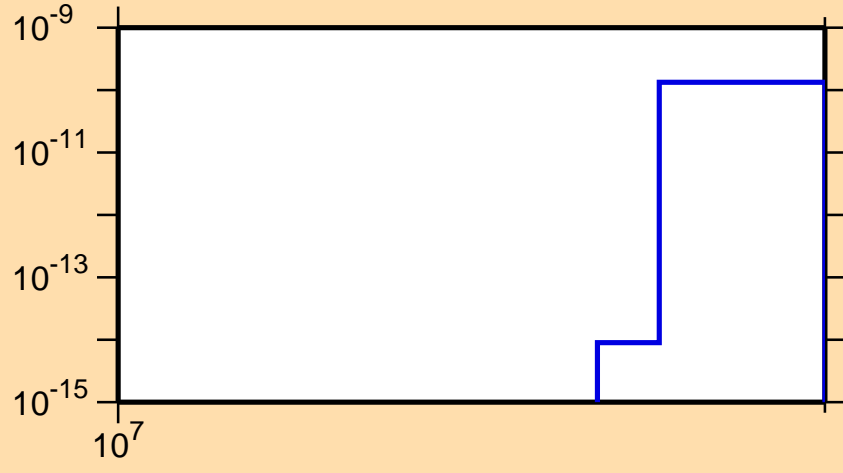
\sigma vs. E for ^{75}\text{Rb} (mt 34)
