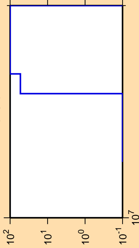
\Delta\sigma/\sigma vs. E for ^{75}\text{Rb}(n,pt)
