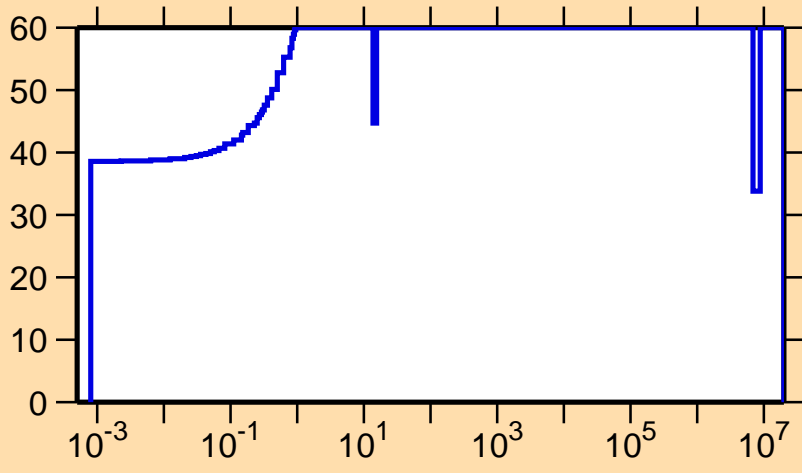
\Delta\sigma/\sigma vs. E for ^{75}\text{Rb}(n,\gamma)
