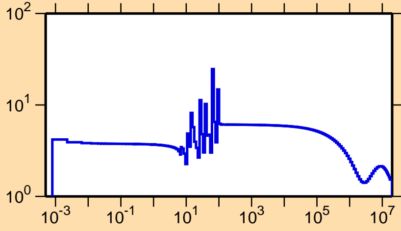
\sigma vs. E for ^{75}\text{Rb}(n,\text{el.})
