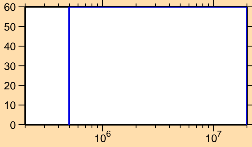
\Delta\sigma/\sigma vs. E for ^{75}\text{Rb}(n,n_1)
