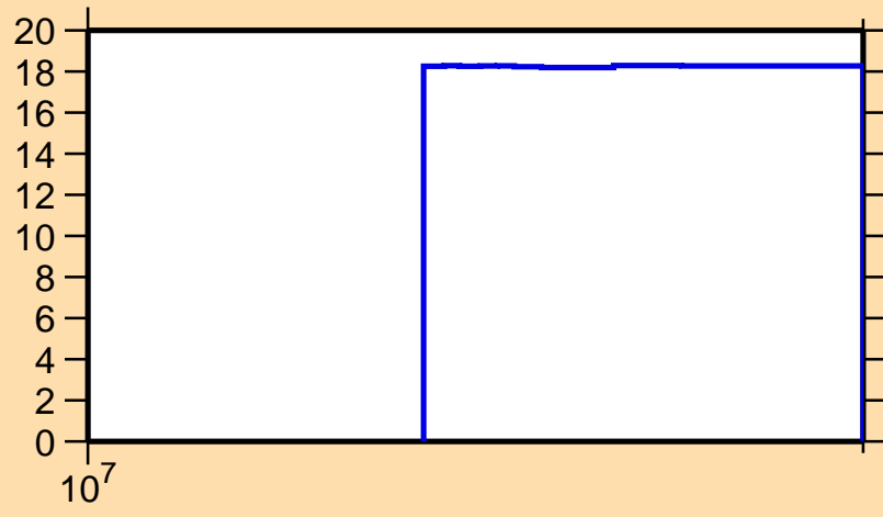
\Delta\sigma/\sigma vs. E for ^{75}\text{Rb}(n,\text{nonel.})
