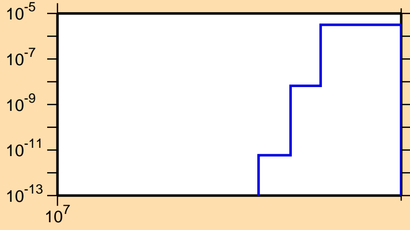
\sigma vs. E for ^{75}\text{Rb}(n,pt)
