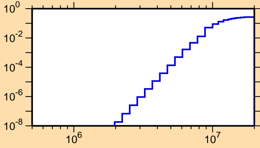
\sigma vs. E for ^{75}\text{Rb}(n,p\alpha)
