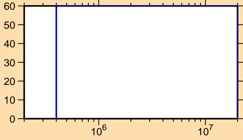
\Delta\sigma/\sigma vs. E for ^{75}\text{Rb}(n,n\text{cont.})
