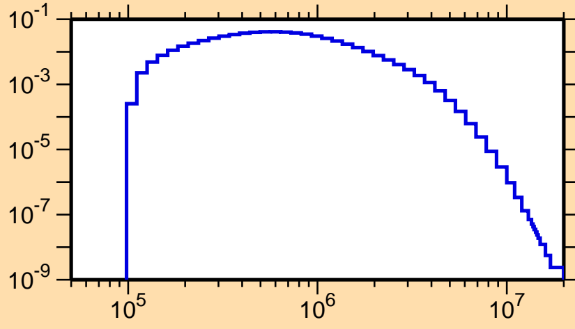
\sigma vs. E for ^{78}\text{Rb}(n,n_2)
