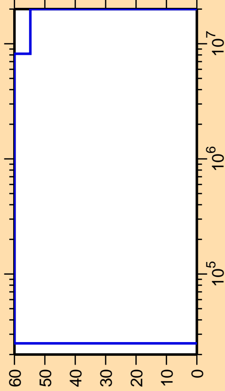
\Delta\sigma/\sigma vs. E for ^{78}\text{Rb}(n,\text{inel.})
