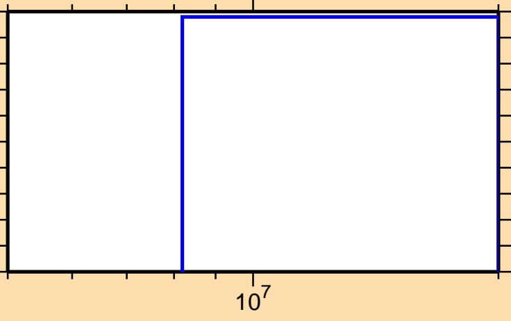
\sigma vs. E for ^{78}\text{Rb}(n,nd)
