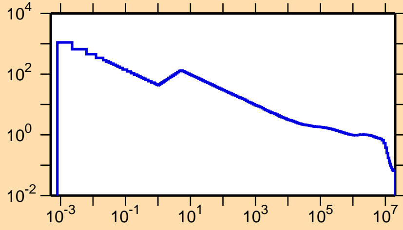
\sigma vs. E for ^{79}\text{Rb}(n,p)
