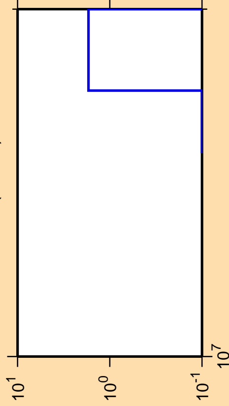
\Delta\sigma/\sigma vs. E for ^{79}\text{Rb} (mt 34)
