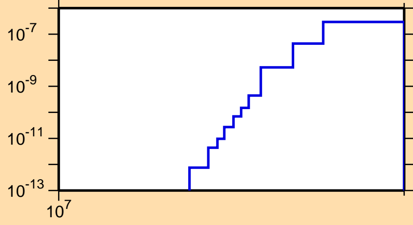
\sigma vs. E for ^{79}\text{Rb} (mt117)
