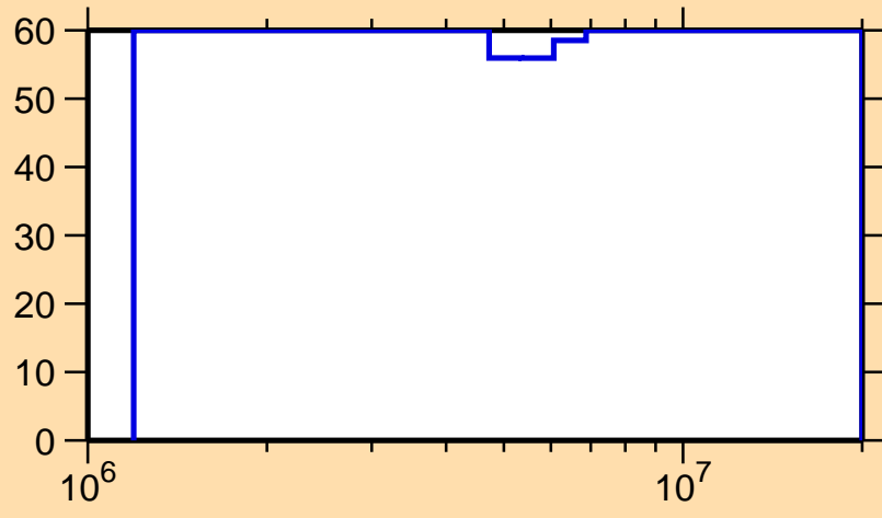
\Delta\sigma/\sigma vs. E for ^{79}\text{Rb}(n,n\text{cont.})
