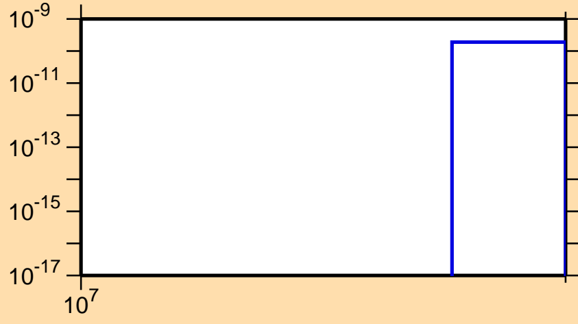
\sigma vs. E for ^{79}\text{Rb}(n,nt)
