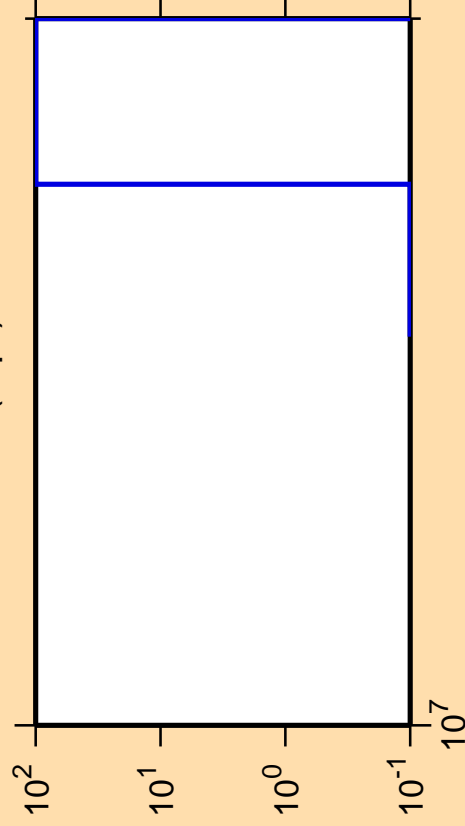
\Delta\sigma/\sigma vs. E for ^{79}\text{Rb}(n,pt)
