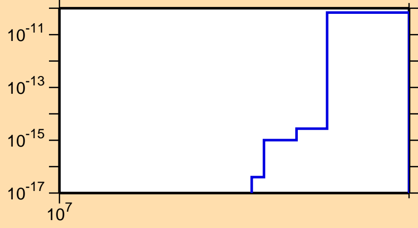
\sigma vs. E for ^{79}\text{Rb}(n,pt)
