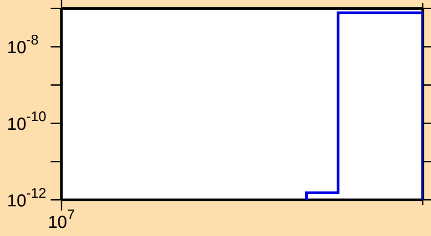
\sigma vs. E for ^{80}\text{Rb}(n,pt)
