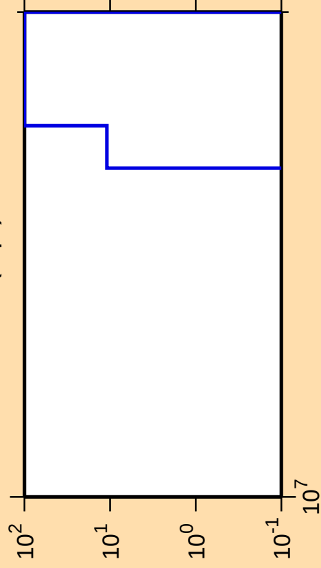
\Delta\sigma/\sigma vs. E for ^{80}\text{Rb}(n,pt)
