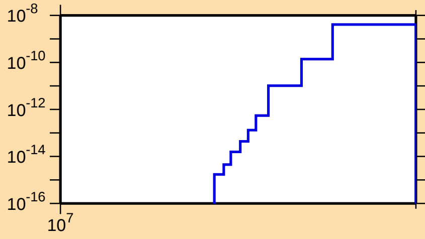
\sigma vs. E for ^{80}\text{Rb}(\text{mt117})
