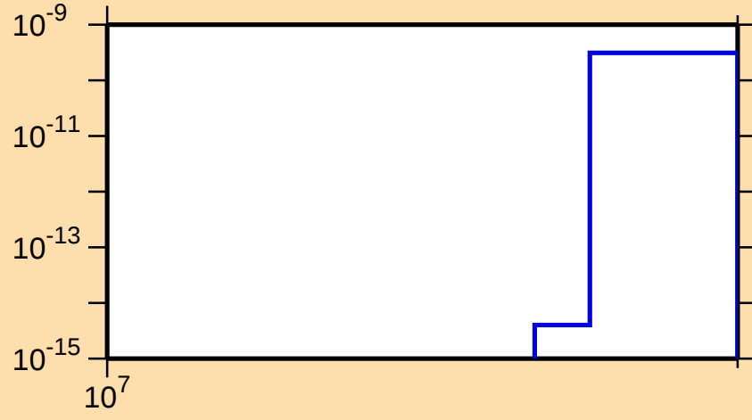
\sigma vs. E for ^{80}\text{Rb} (mt 34)
