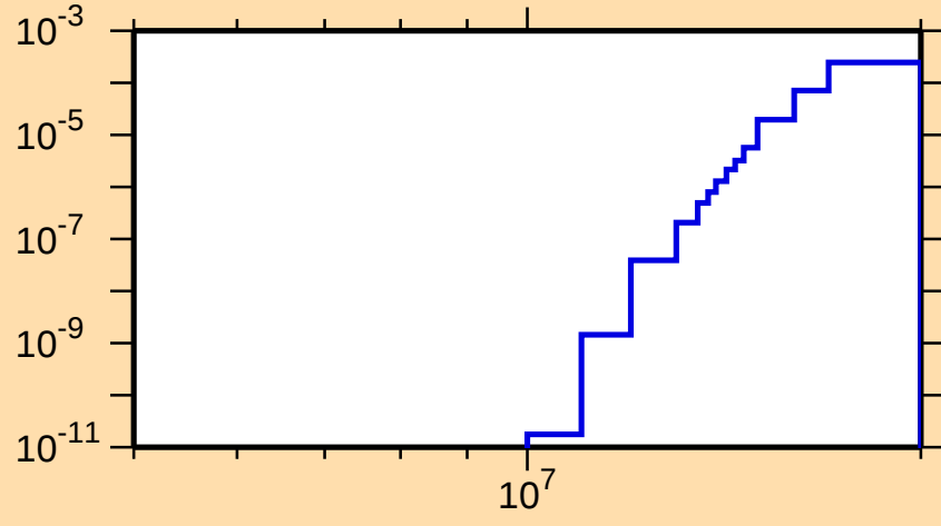
\sigma vs. E for ^{80}\text{Rb}(n,\text{He3})
