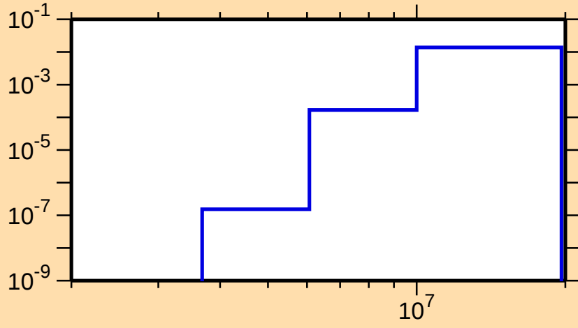
\sigma vs. E for ^{80}\text{Rb}(n,d)
