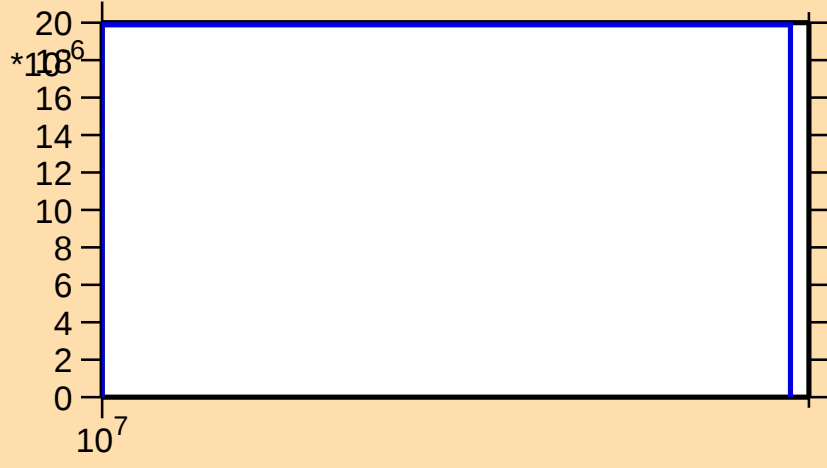
\sigma vs. E for ^{80}\text{Rb}(n,\text{nd})
