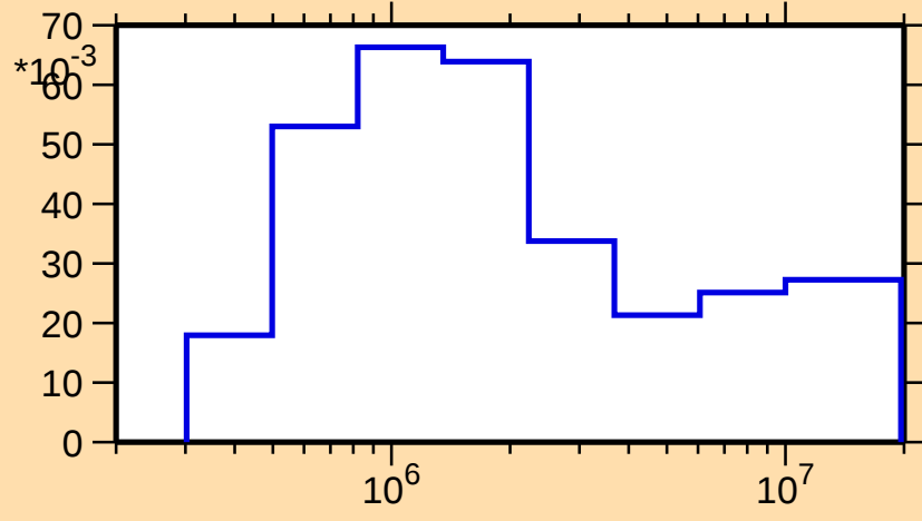
\sigma vs. E for ^{80}\text{Rb}(n,n_3)
