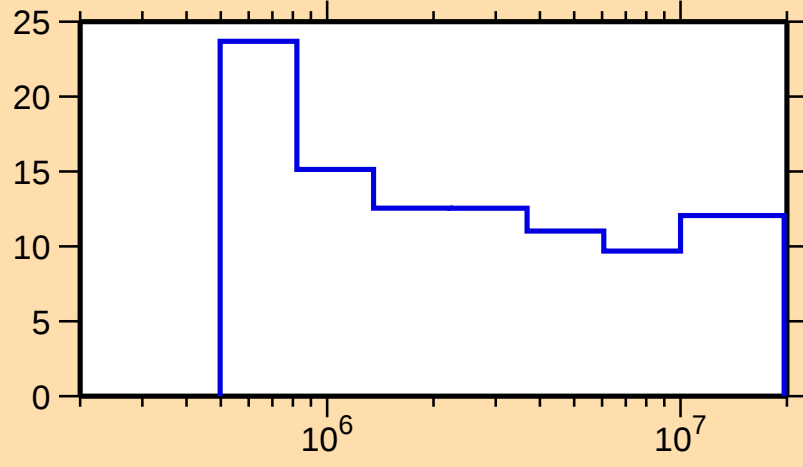
\Delta\sigma/\sigma vs. E for ^{80}\text{Rb}(n,n\text{nonel.})
