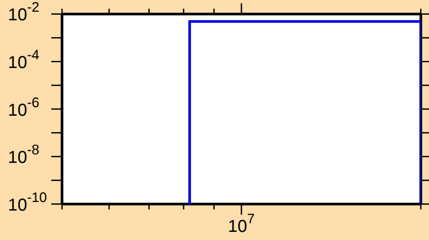
\sigma vs. E for ^{80}\text{Rb}(n,n\alpha)
