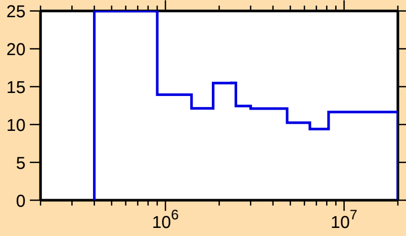
\Delta\sigma/\sigma vs. E for ^{80}\text{Rb}(n,n\text{oncl.})
