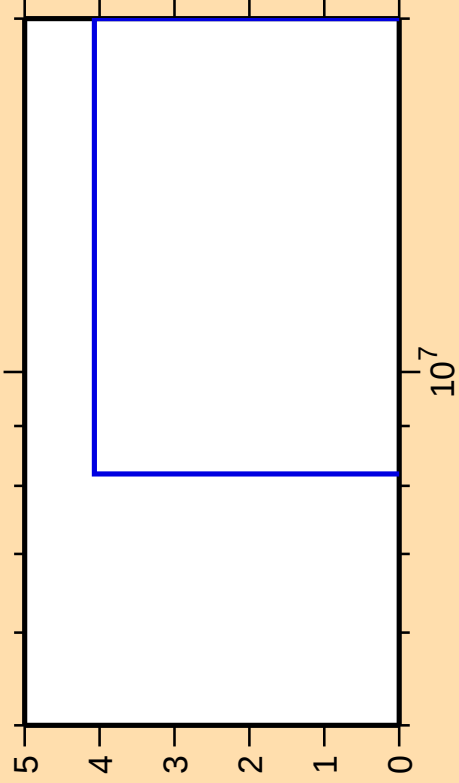
\Delta\sigma/\sigma vs. E for ^{80}\text{Rb}(n,nt)
