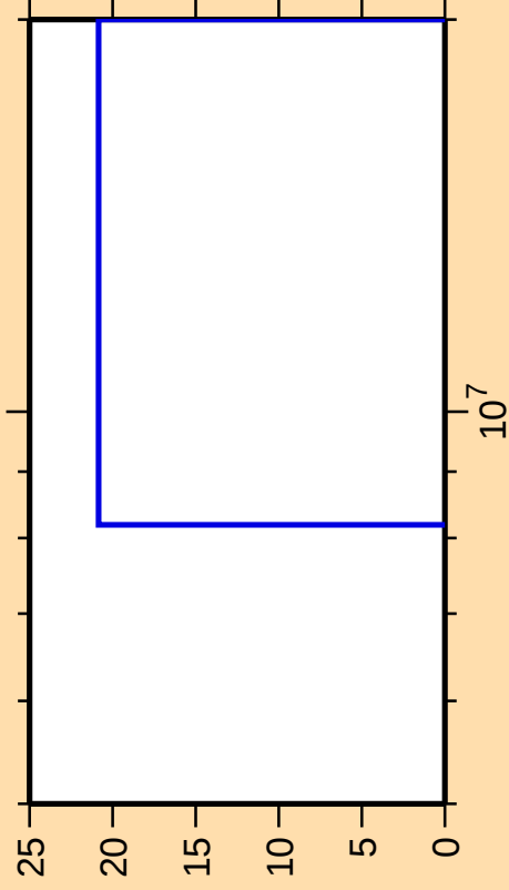
\Delta\sigma/\sigma vs. E for ^{80}\text{Rb}(\text{mt } 34)
