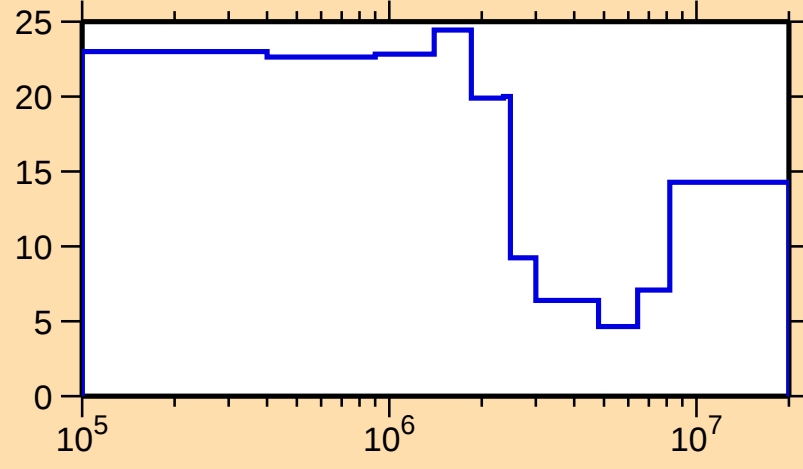
\Delta\sigma/\sigma vs. E for ^{80}\text{Rb}(n,\text{tot.})
