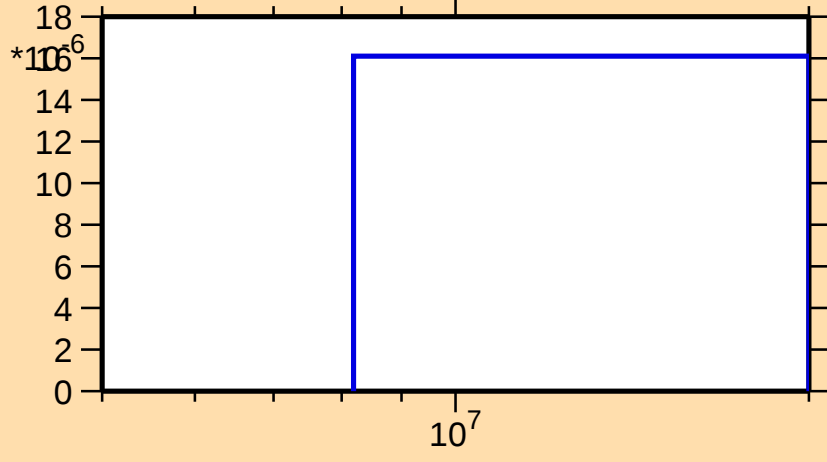
\sigma vs. E for ^{80}\text{Rb}(n,\text{nd})
