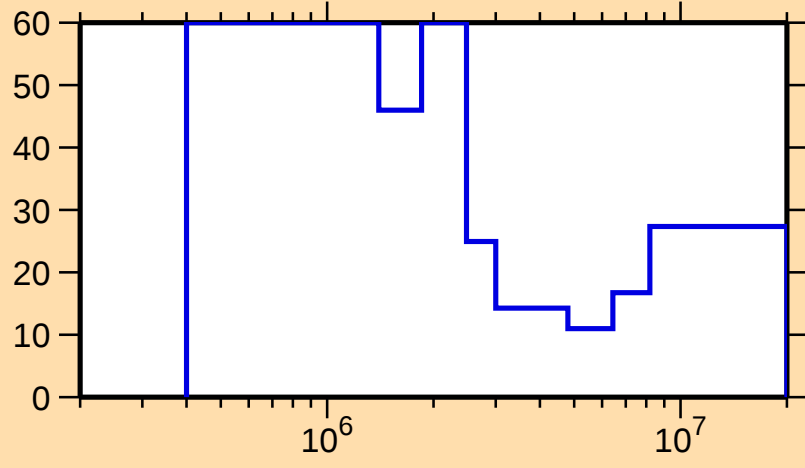
\Delta\sigma/\sigma vs. E for ^{80}\text{Rb}(n,n\text{cont.})
