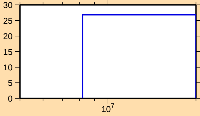
\Delta\sigma/\sigma vs. E for ^{80}\text{Rb}(n,\text{inel.})
