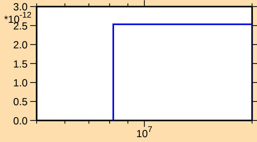
\sigma vs. E for ^{80}\text{Rb}(\text{mt } 34)
