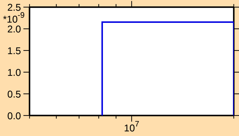
\sigma vs. E for ^{80}\text{Rb}(\text{mt } 45)
