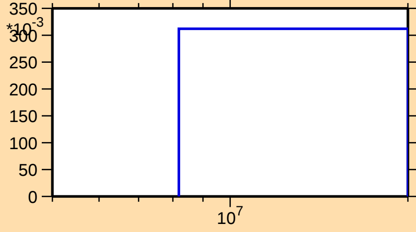
\sigma vs. E for ^{80}\text{Rb}(n,2n)
