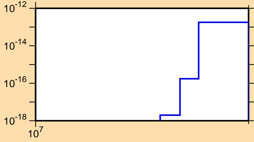
\sigma vs. E for ^{81}\text{Rb}(n,2n\alpha)
