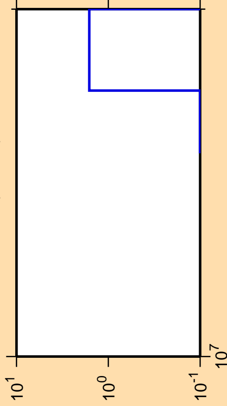
\Delta\sigma/\sigma vs. E for ^{81}\text{Rb}(n,2n\alpha)
