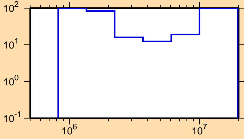
\Delta\sigma/\sigma vs. E for ^{81}\text{Rb}(n,n\text{cont.})
