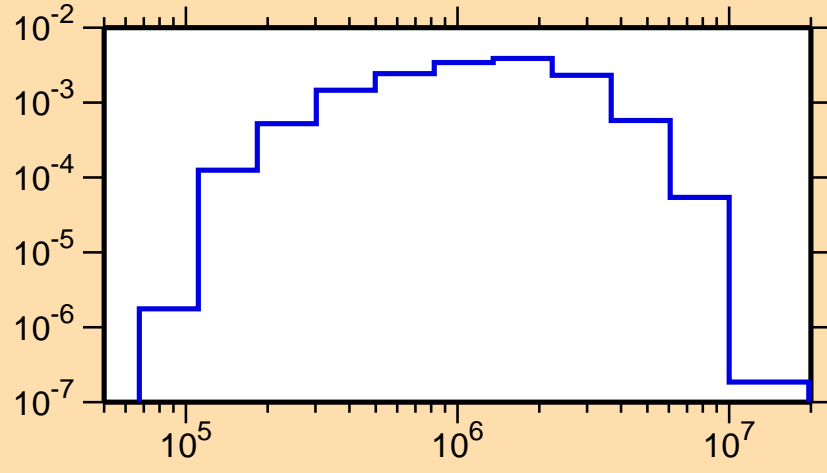
\sigma vs. E for ^{81}\text{Rb}(n,n_3)
