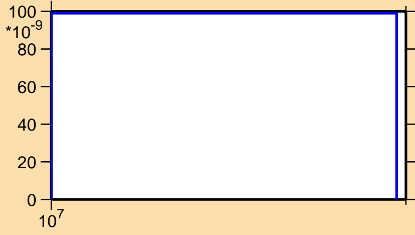
\sigma vs. E for ^{81}\text{Rb}(n,\text{nd})
