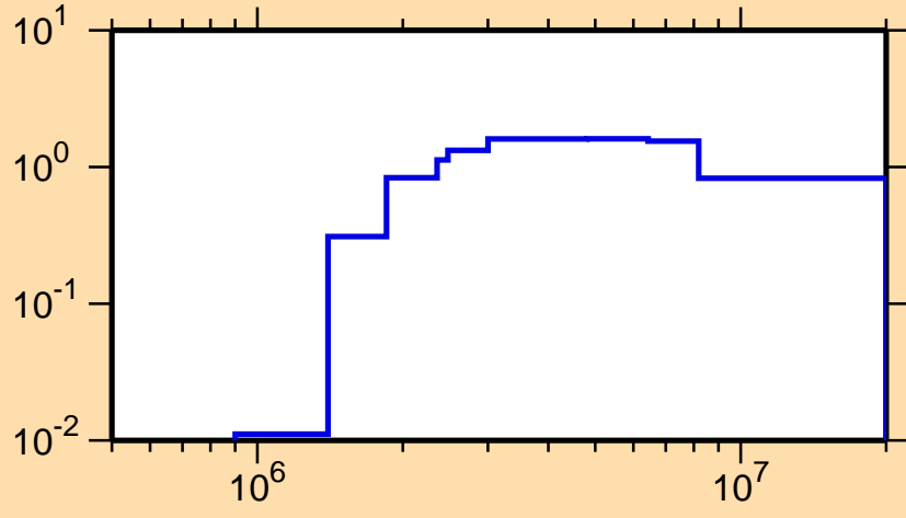
\sigma vs. E for ^{81}\text{Rb}(n,n\text{cont.})
