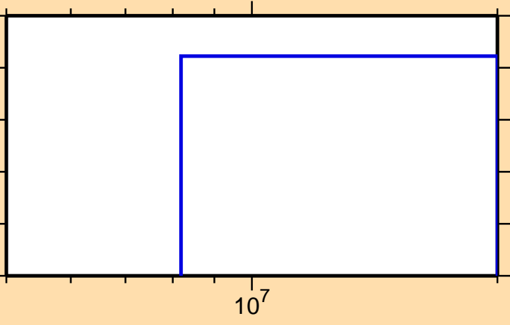
\sigma vs. E for ^{81}\text{Rb}(n,2np)
