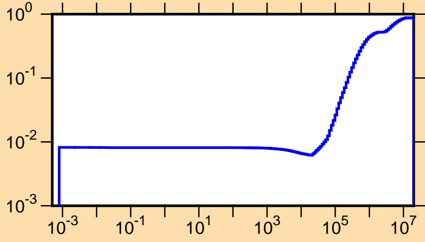
\mu vs. E for ^{82}\text{Rb}(\text{mt251})
